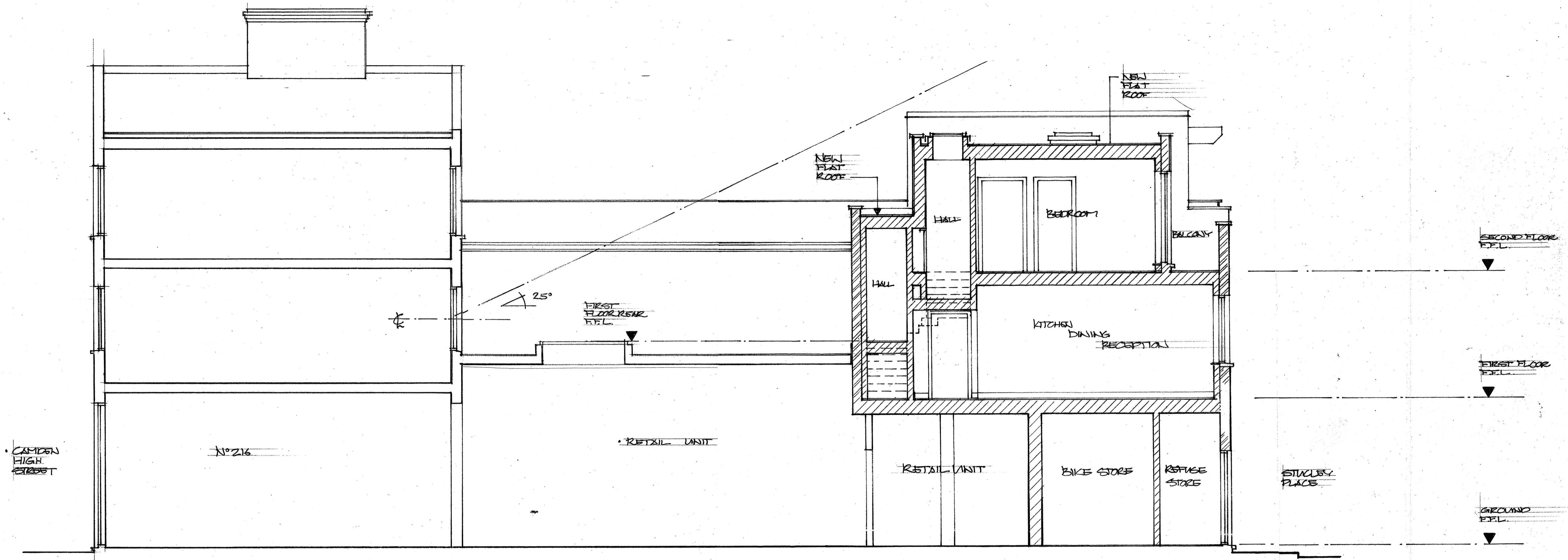
PROPOSED SECTION \text{D/10}
