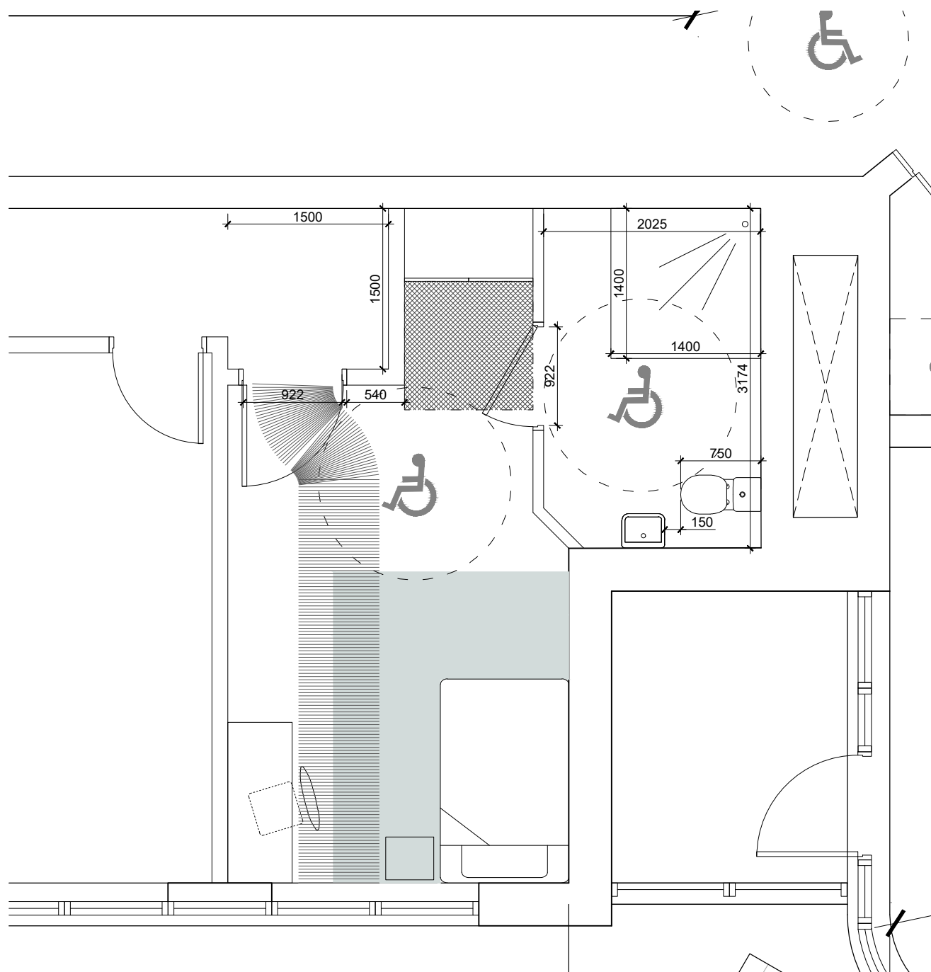
02 Wheelchair Room - Cluster A Plan 1:50
