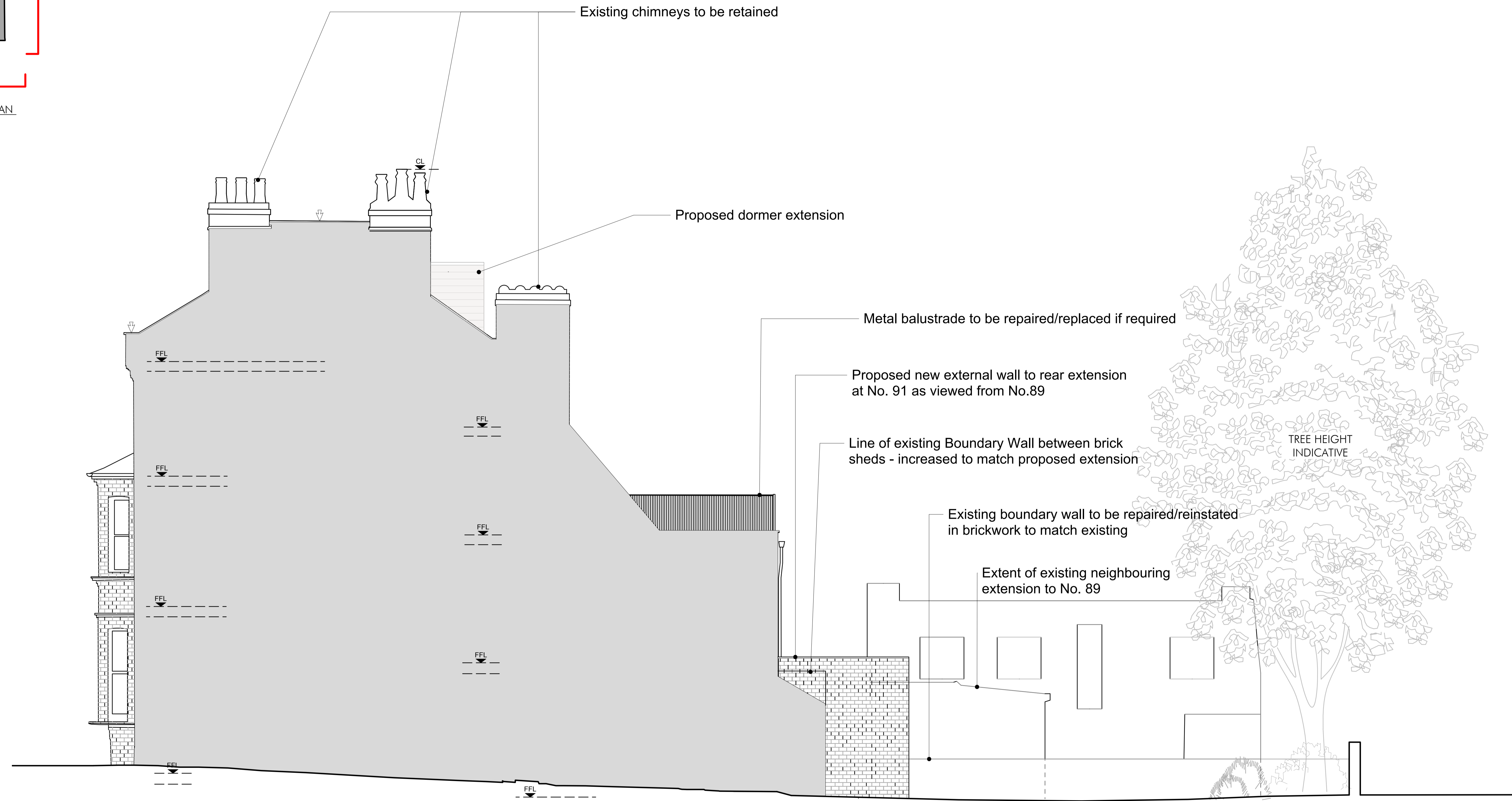
Proposed Side Elevation D Scale: 100@A3
