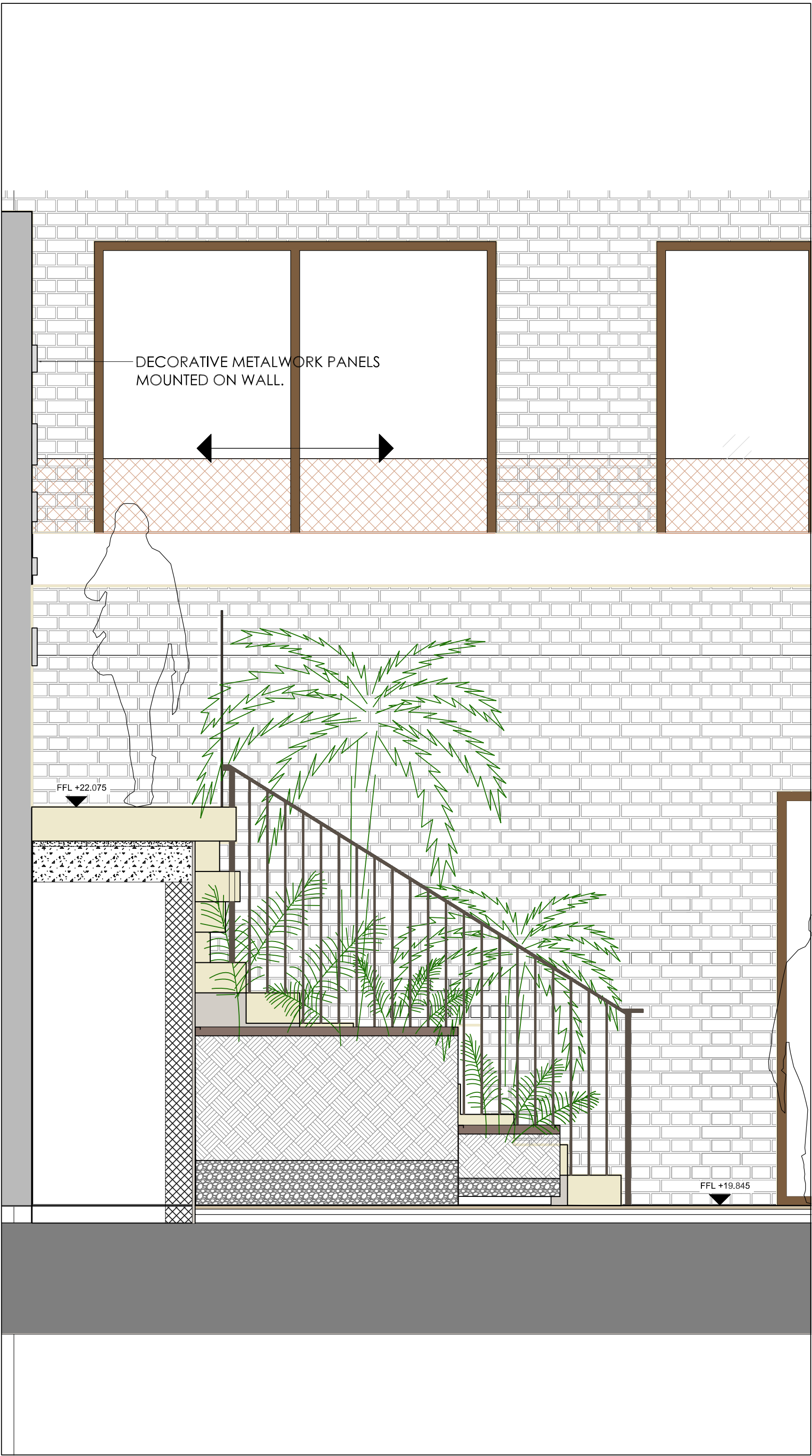
02 Decorative metal panels on rendered wall - Section - scale 1:20@ A1 140 Basement Gardens - B1
