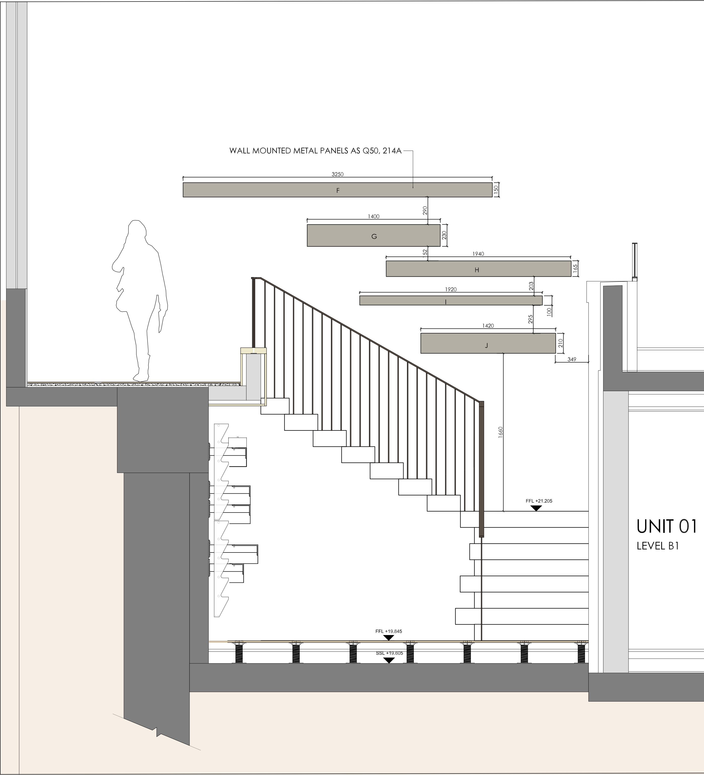
01 Decorative metal panels on rendered wall - Elevation - scale 1:20@ A1 140 Basement Gardens - B1
