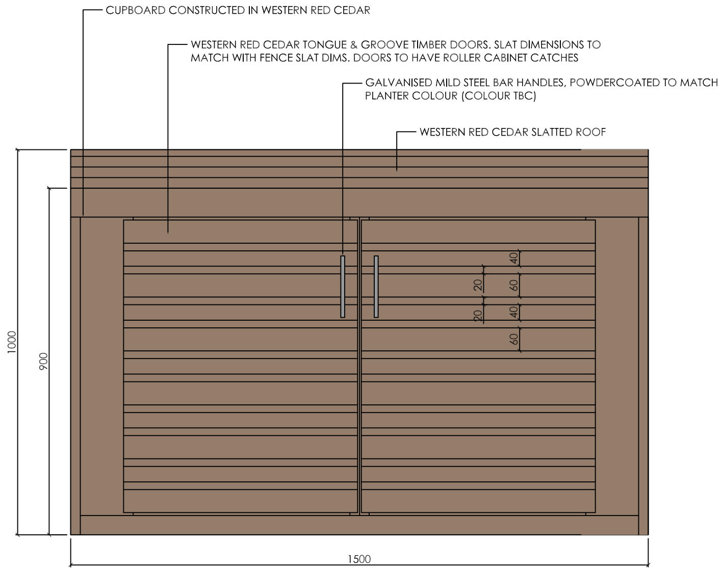
01 Storage cupboard (style guide) - scale 1:10@ A3 450 Aldwych Mews
