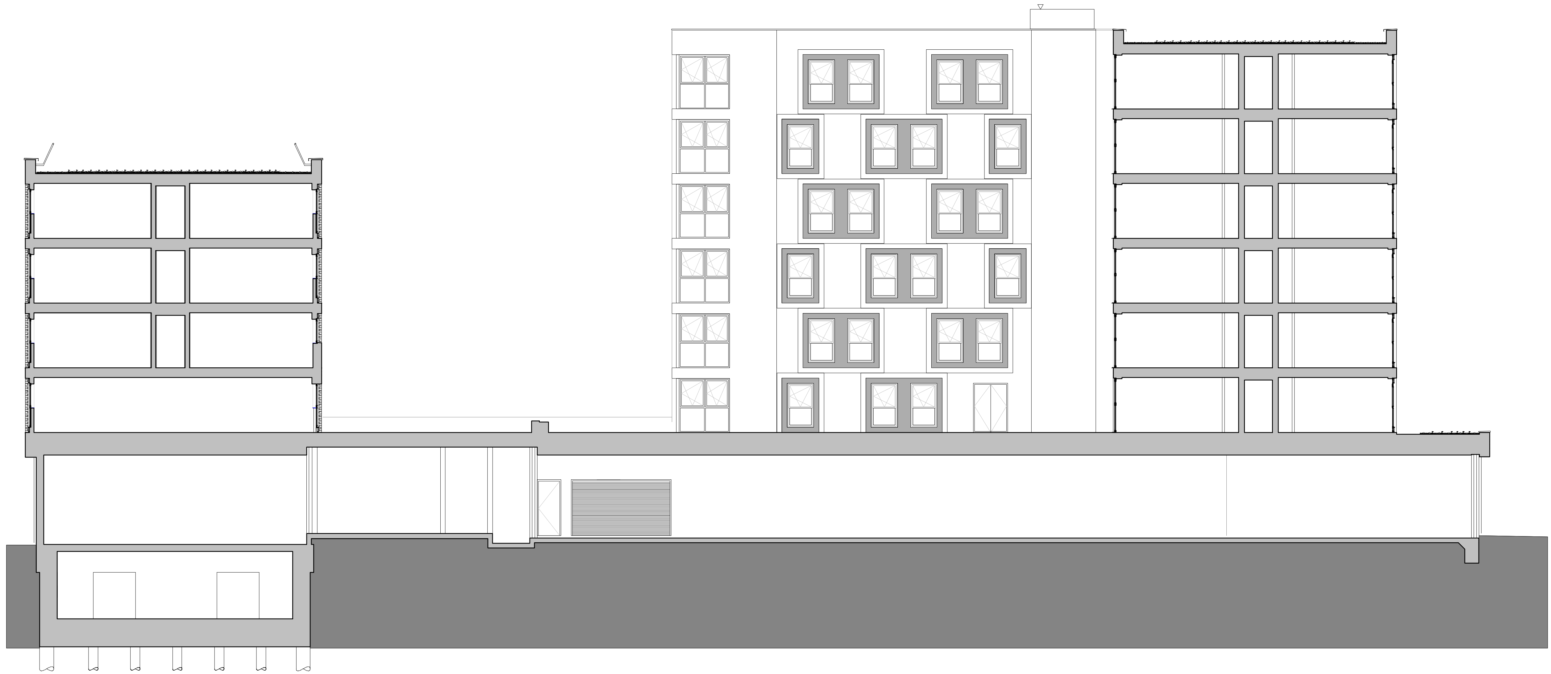
1 Existing Section 4-4 Scale 1 : 200 @ A3
