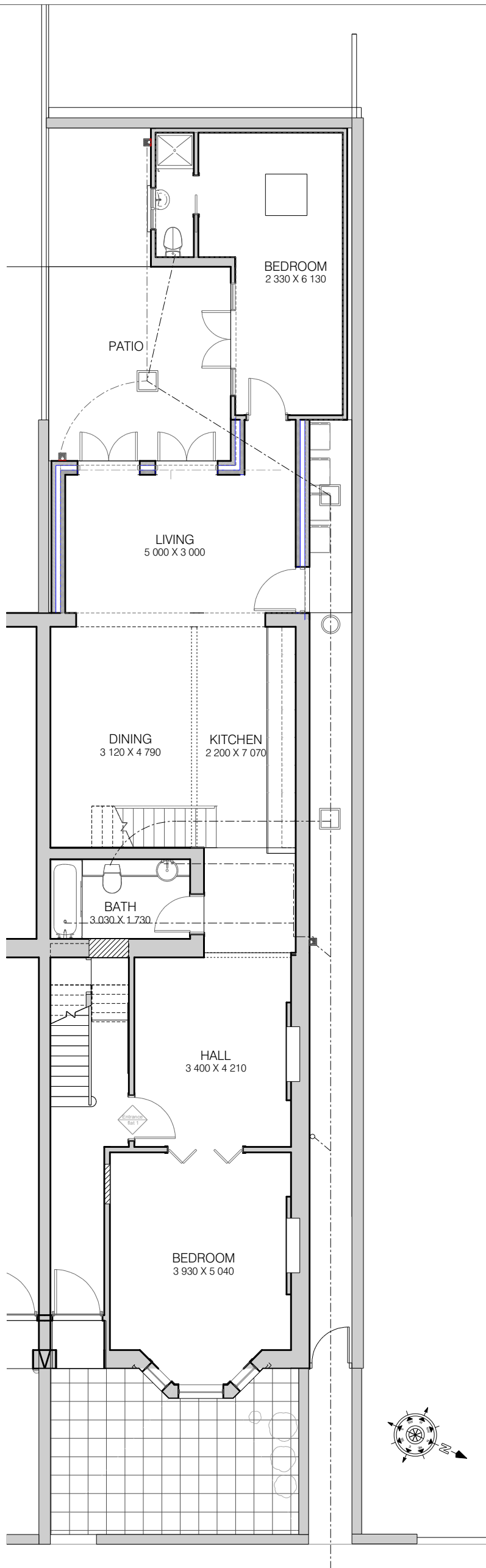
Proposed ground floor plan
