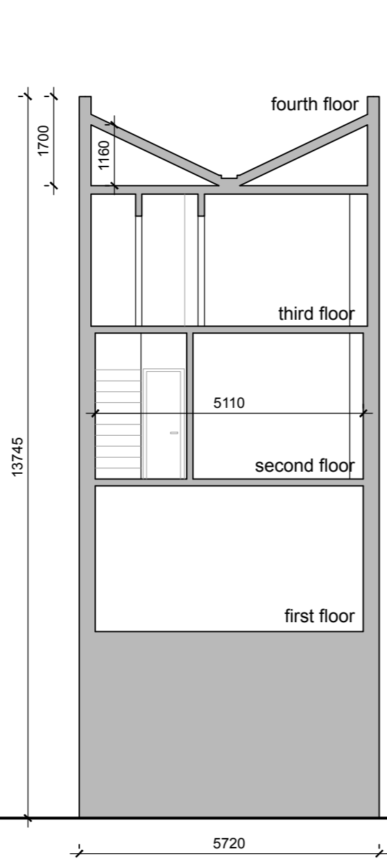
EXISTING SITUATION_CROSS SECTION 44 FALKLAND ROAD
