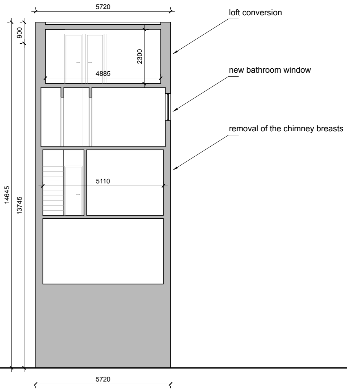
DESIGN PROPOSAL_CROSS SECTION 44 FALKLAND ROAD
