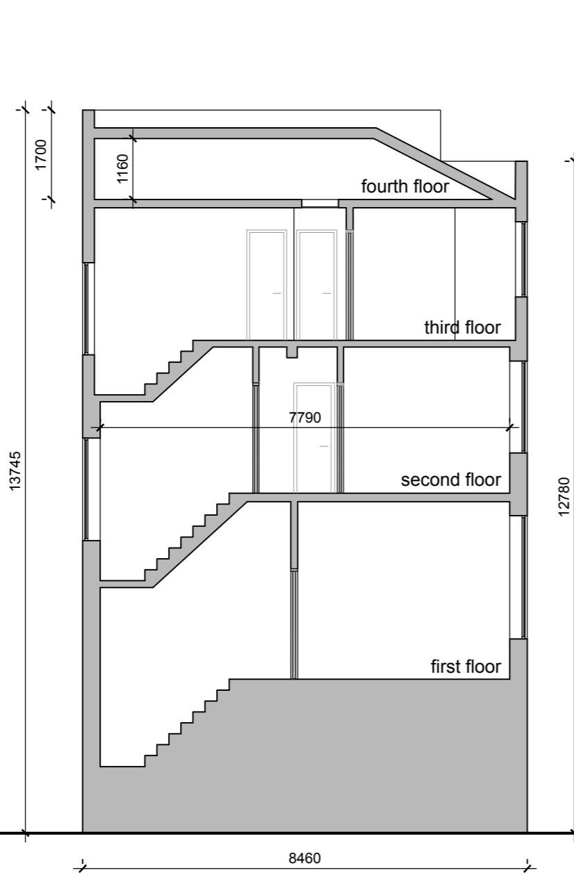
EXISTING SITUATION_LONGITUDINAL SECTION 44 FALKLAND ROAD
