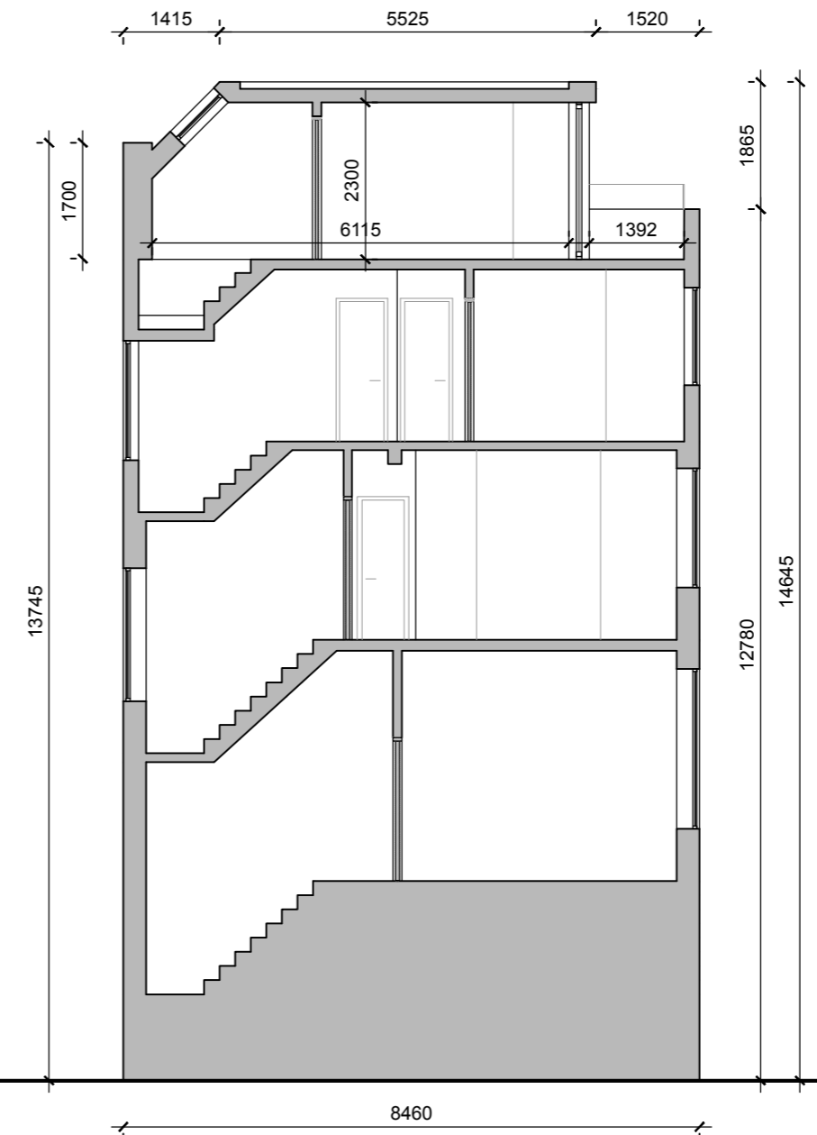
DESIGN PROPOSAL_LONGITUDINAL SECTION 44 FALKLAND ROAD
