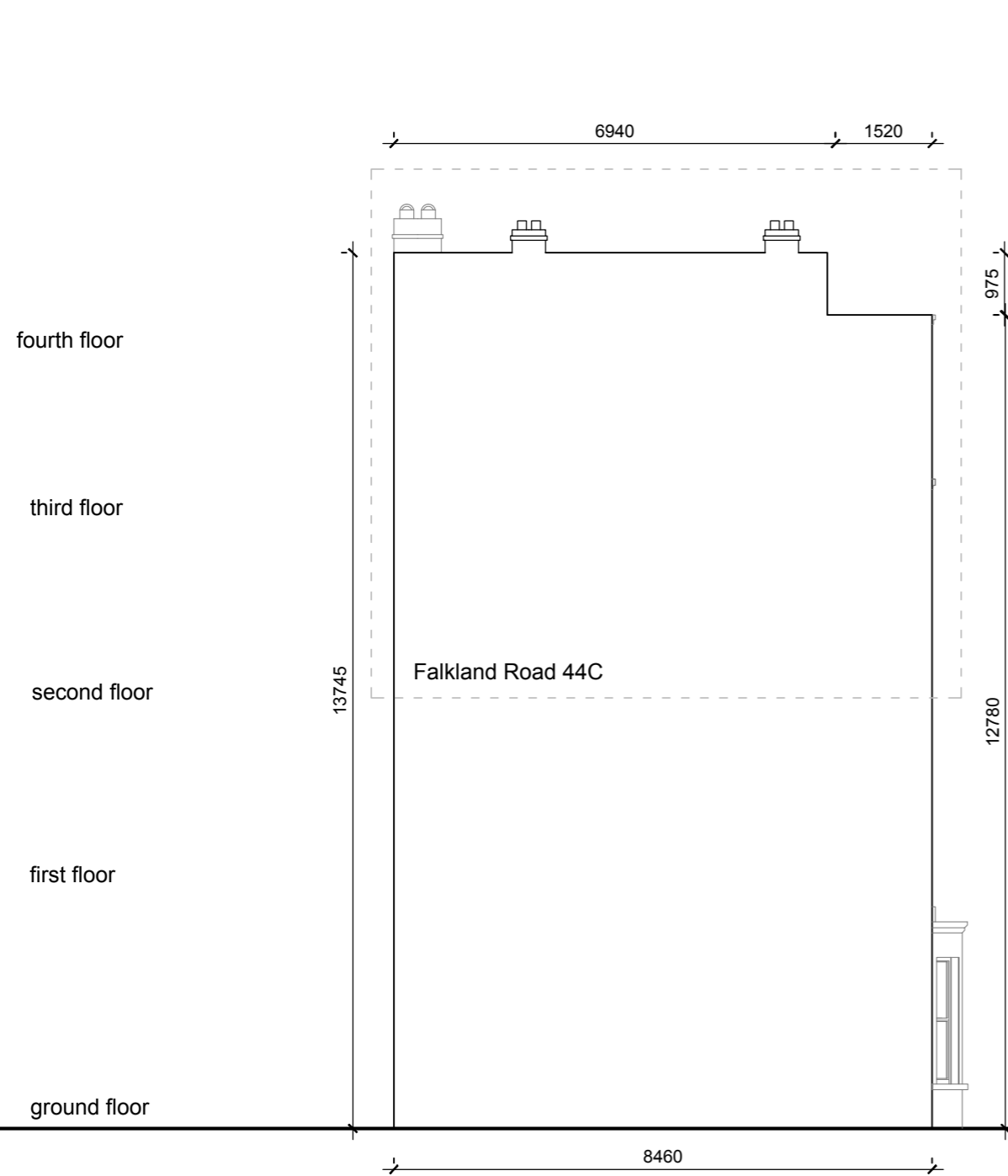
EXISTING SITUATION _SIDE ELEVATION 44 FALKLAND ROAD
