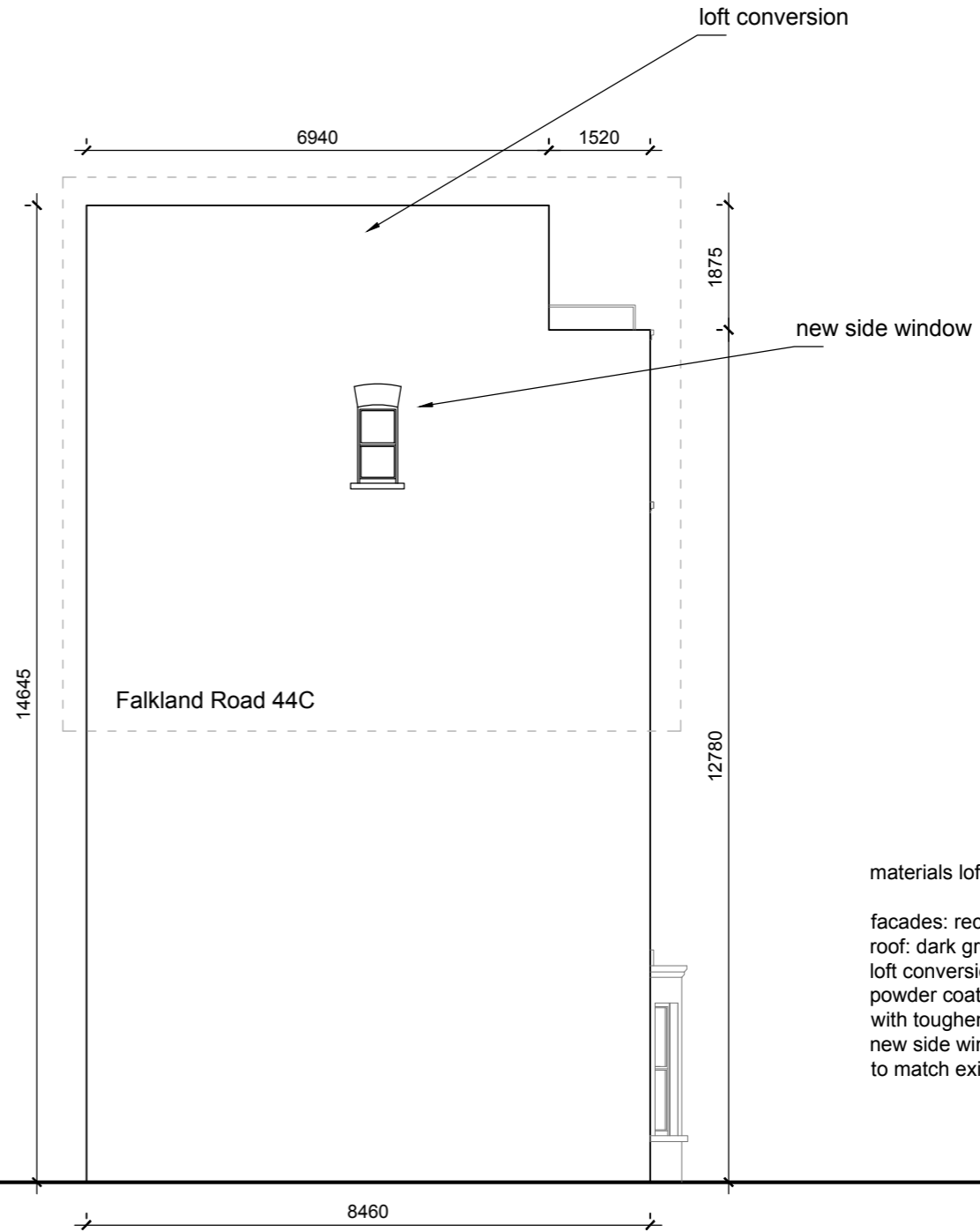
DESIGN PROPOSAL _SIDE ELEVATION 44 FALKLAND ROAD
