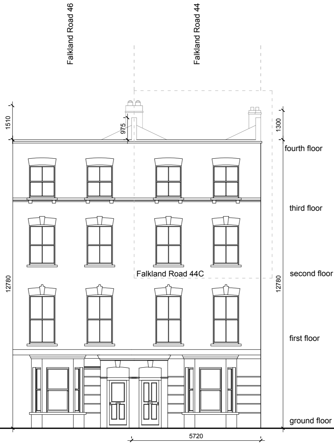
EXISTING SITUATION_FRONT ELEVATION 44 FALKLAND ROAD
