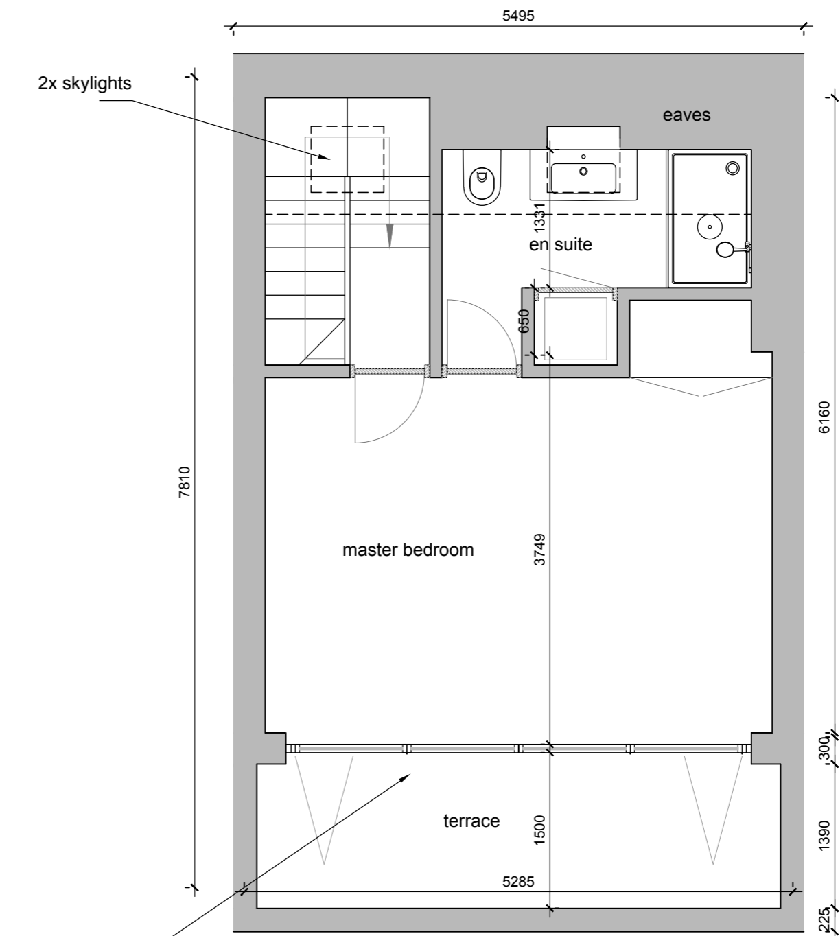
DESIGN PROPOSAL_FOURTH FLOOR_FLOORPLAN FLAT 44c
