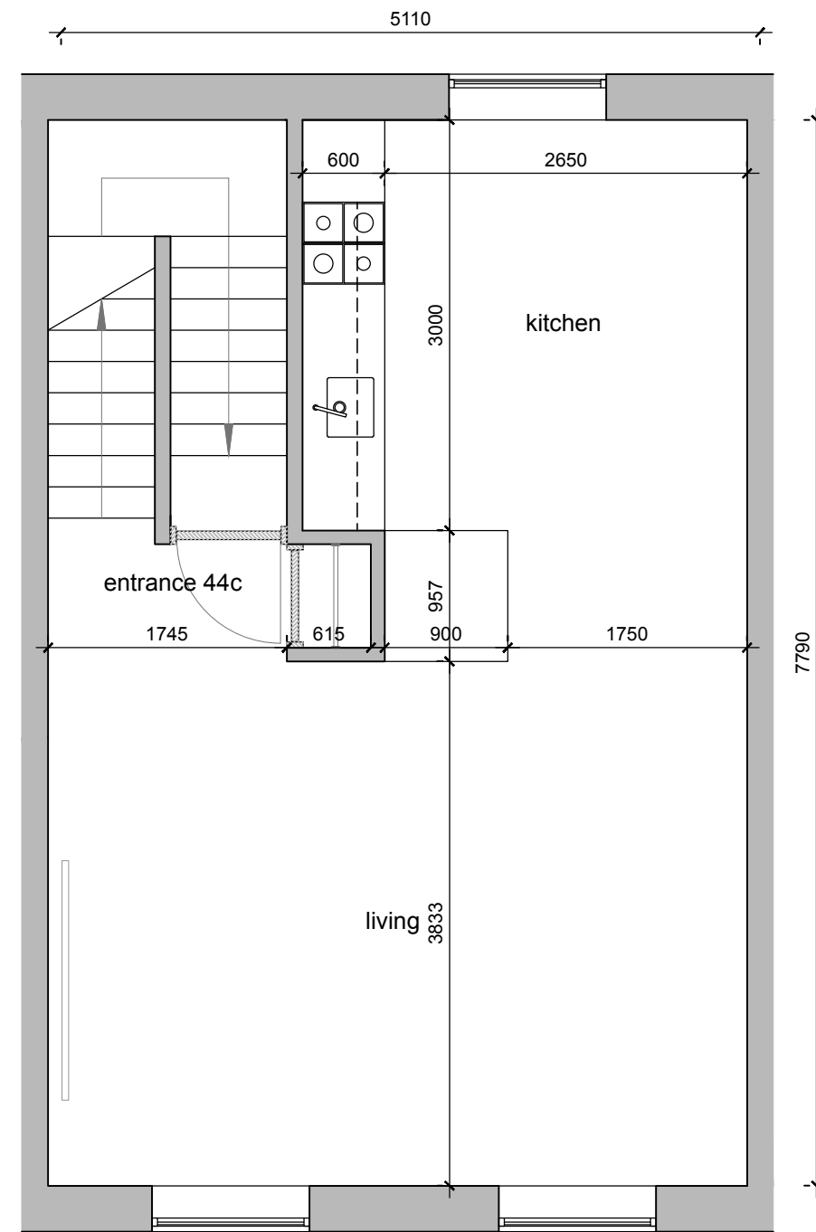
DESIGN PROPOSAL_SECOND FLOOR_FLOORPLAN FLAT 44c
