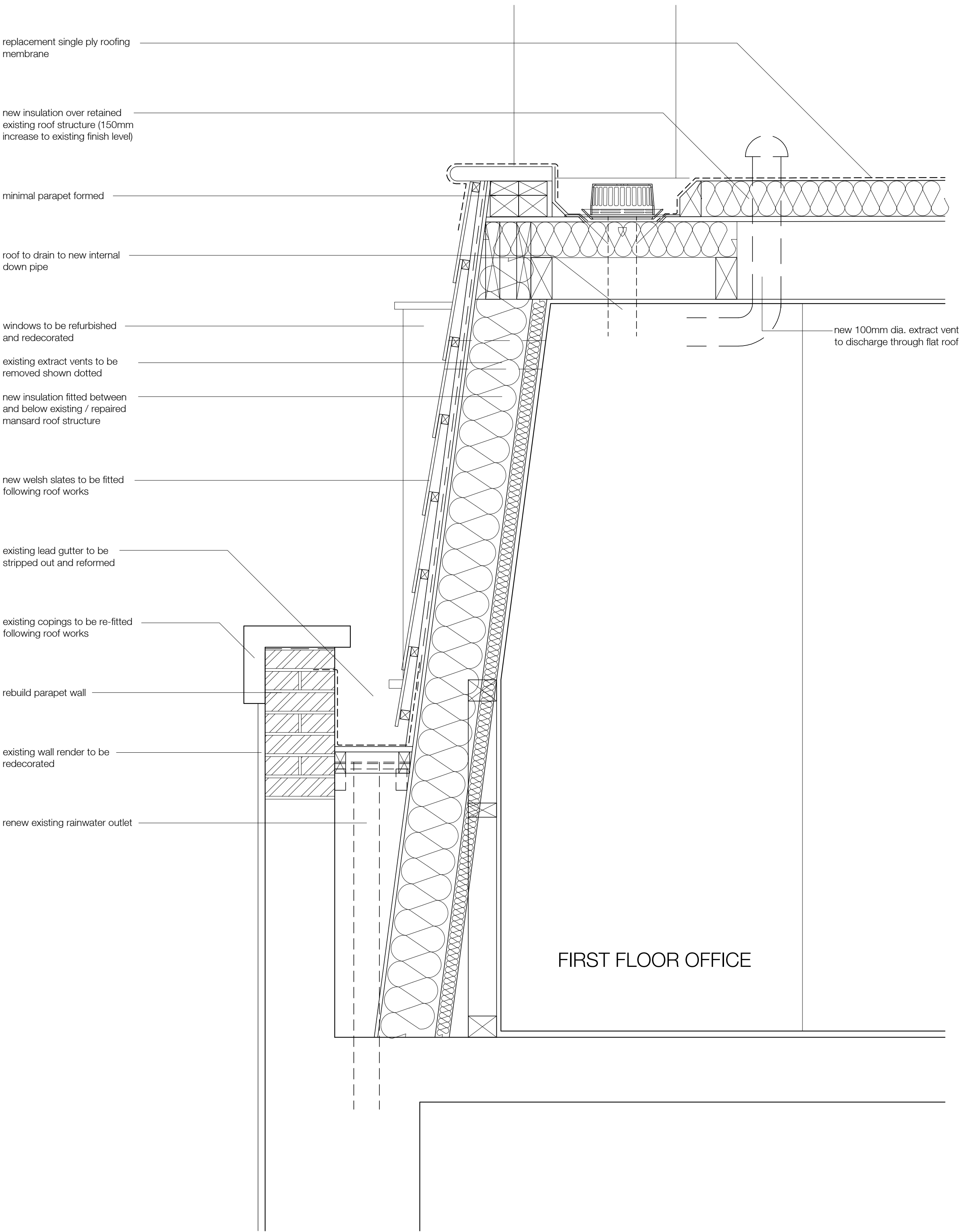
MANSARD ROOF WORKS 1:10
