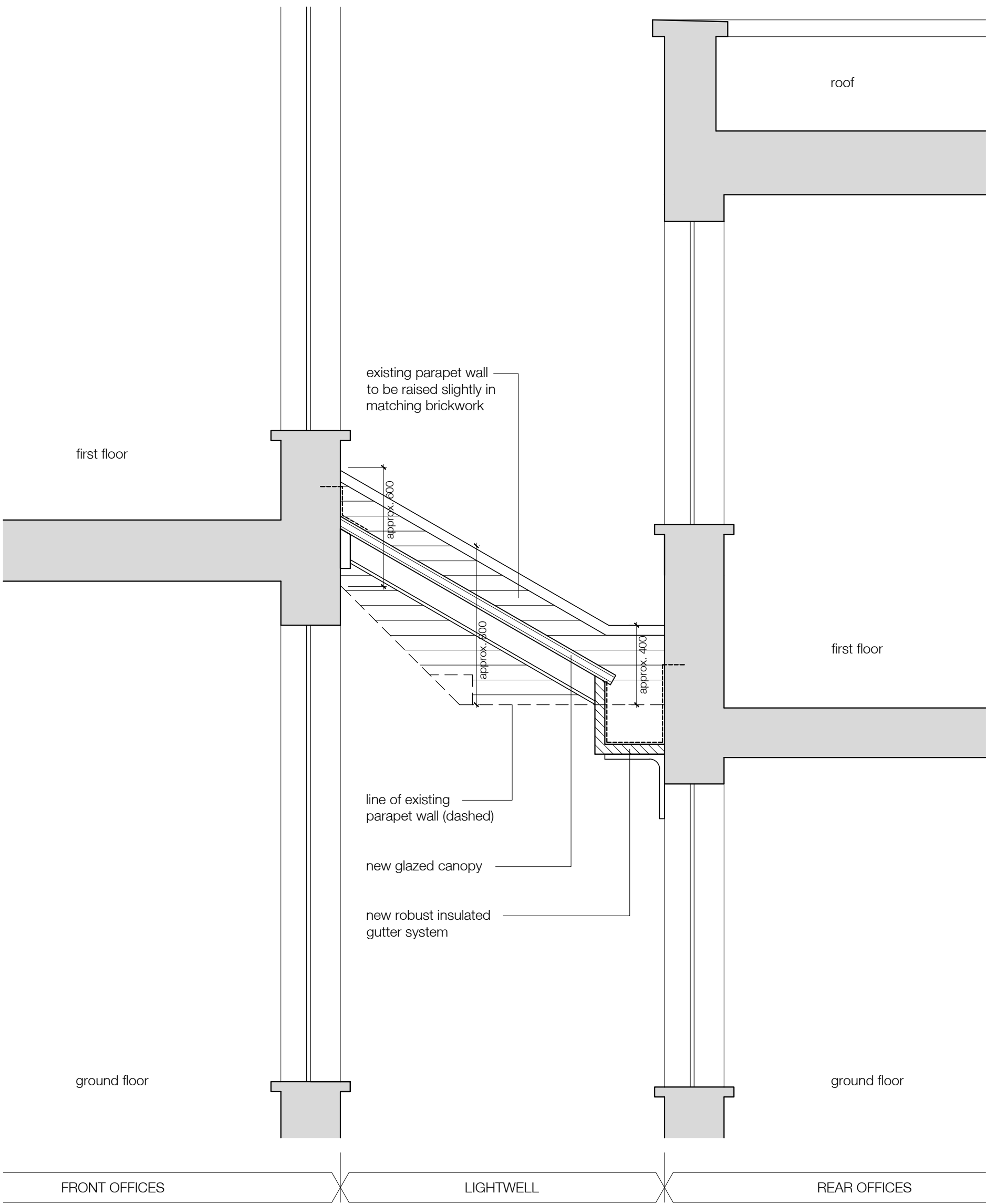
STAIRWELL GLAZING 1:20
