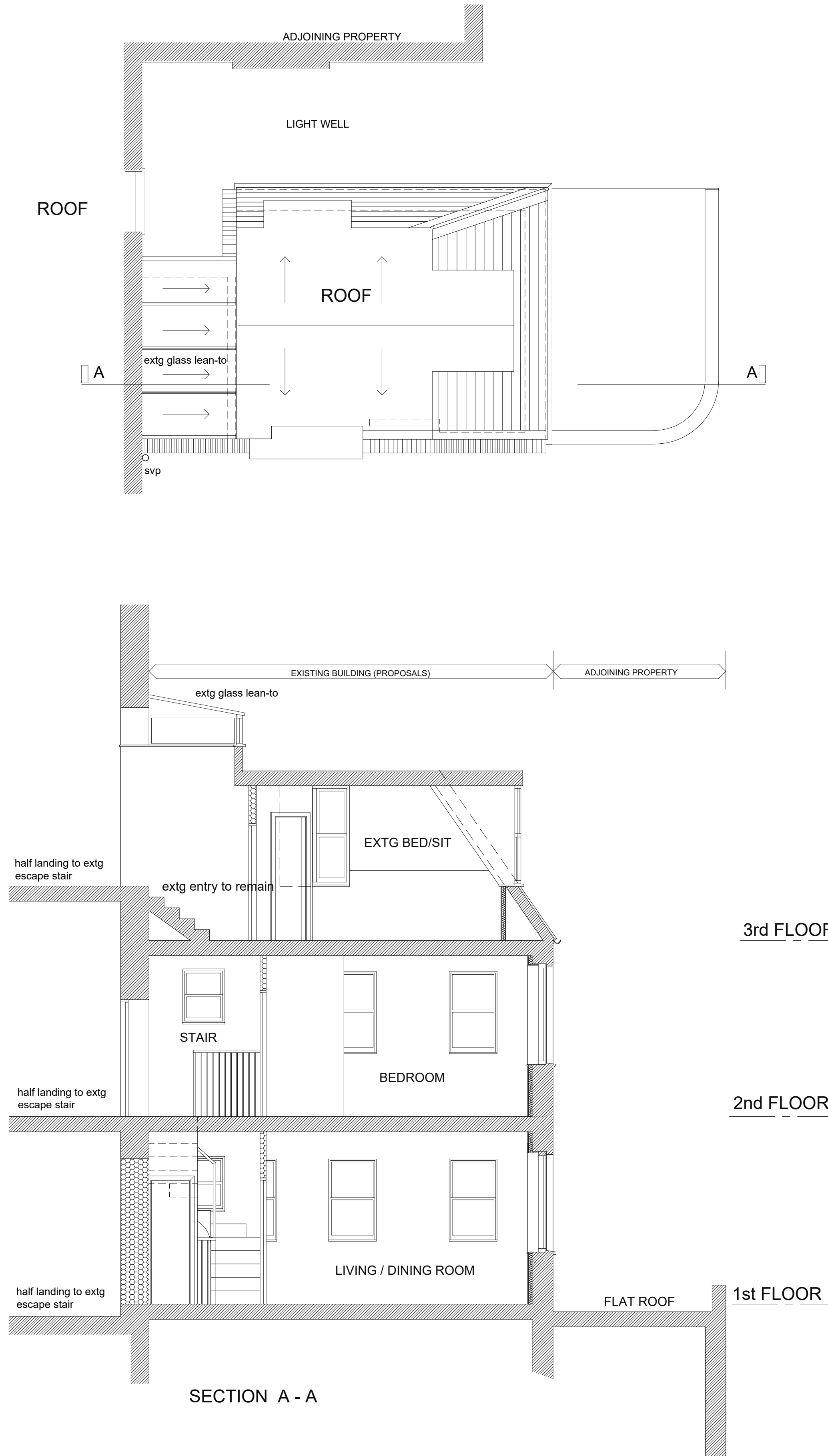
PROPOSED FLOOR PLANS, SECTION & ELEVATION SCALE 1:50@A1 / 1:100@A3 SCALE BAR 1:50@A1 0 1 2 3 4 5 METRES SCALE BAR 1:100@A3 0 1 2 3 4 5 6 7 8 9 10 METRES
