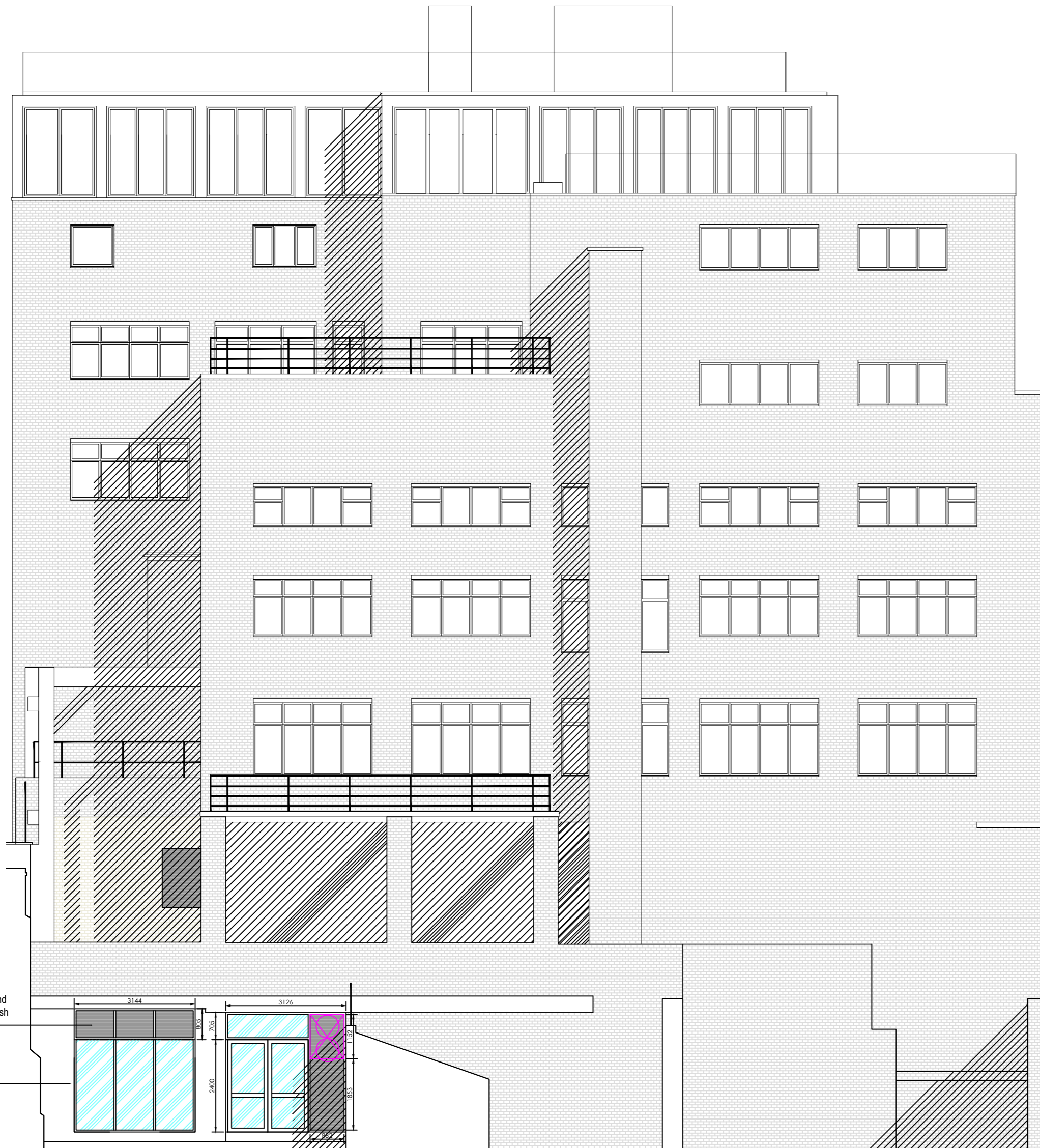
SIDE ELEVATION - A
