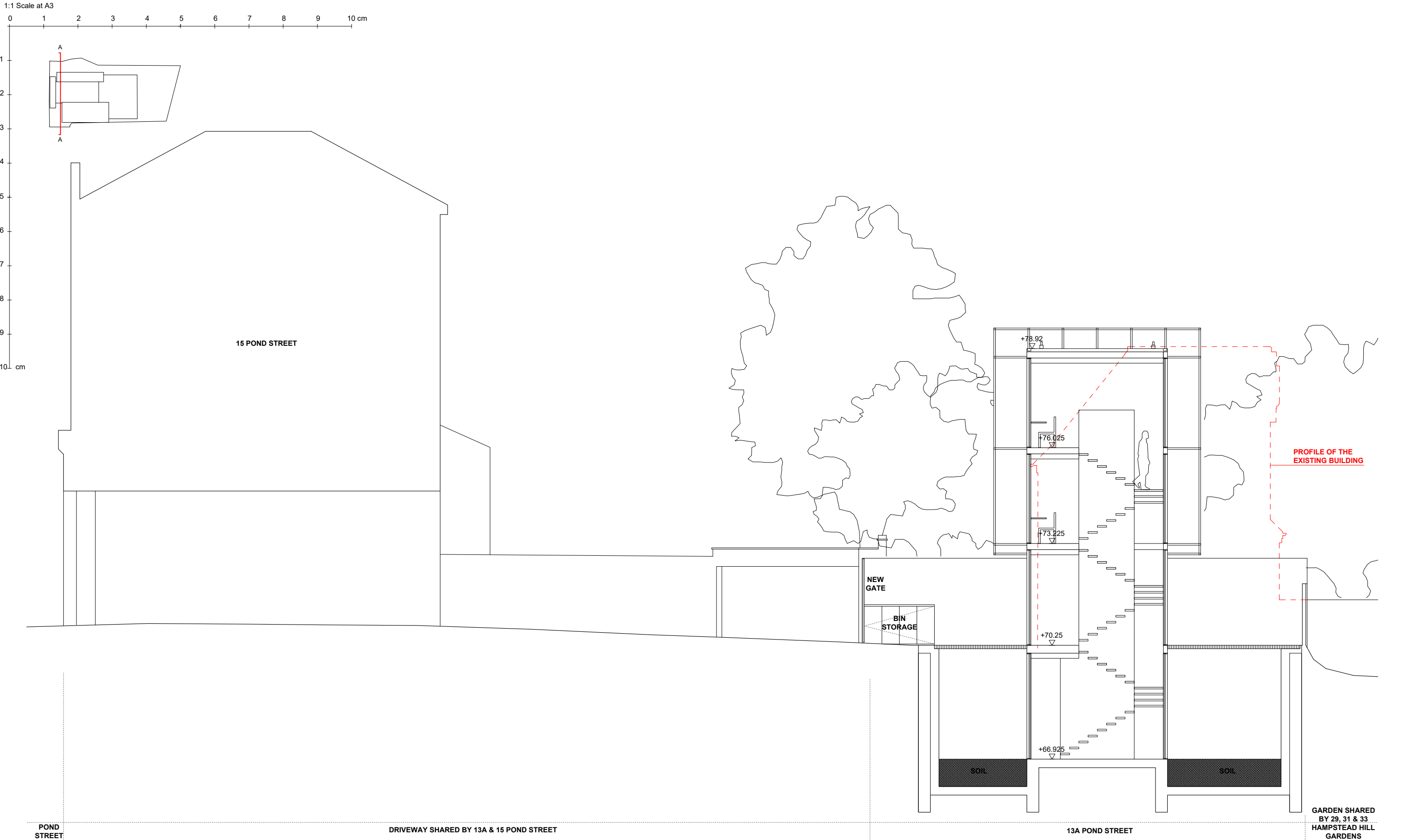
01 Proposed - Section A-A
