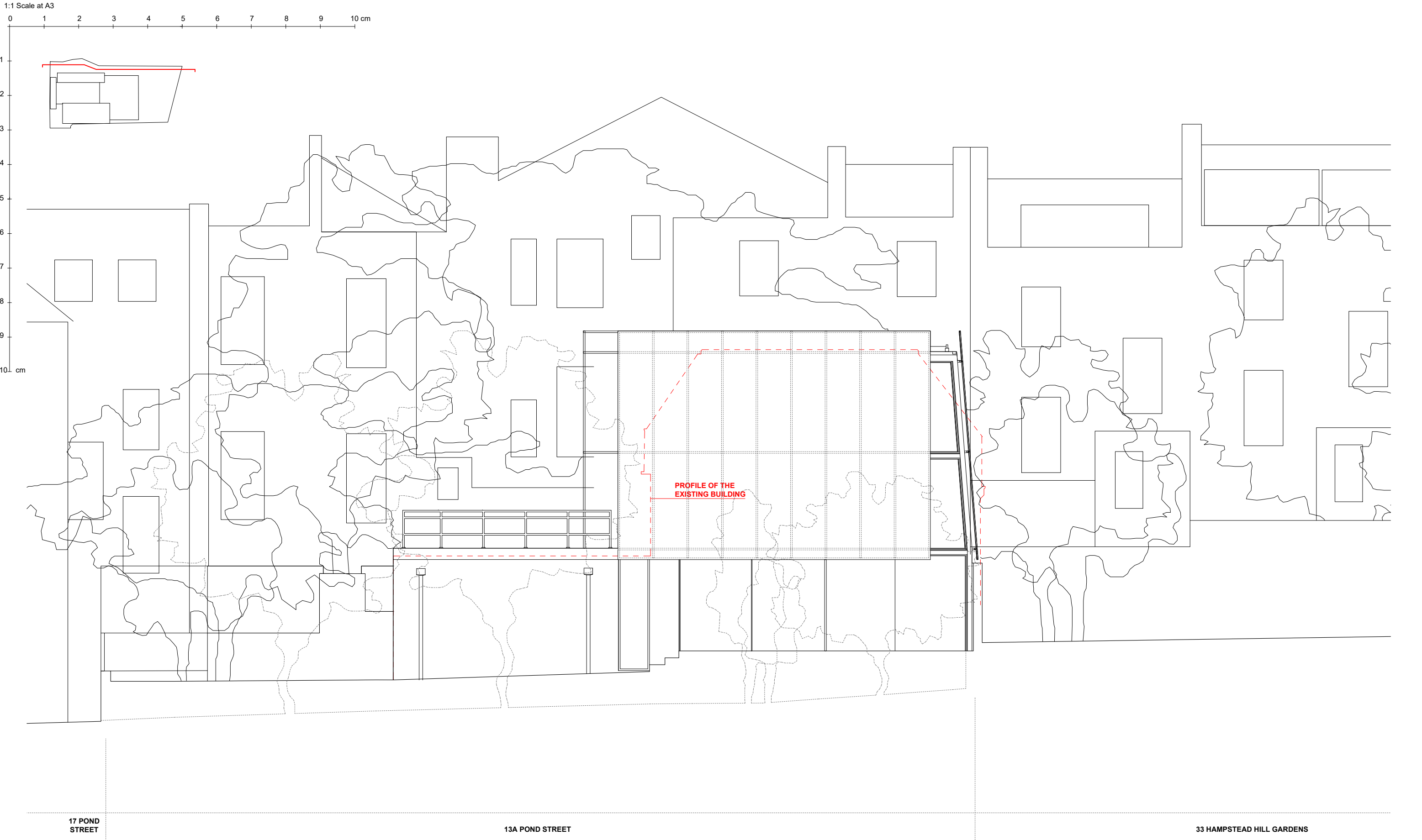
01 Proposed - North Elevation
