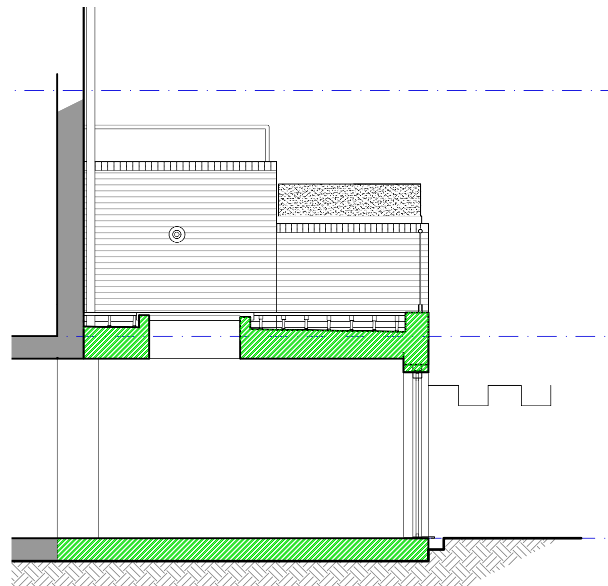
05 West Elevation of East Boundary Wall (Extension #156) PROPOSED 1:50
