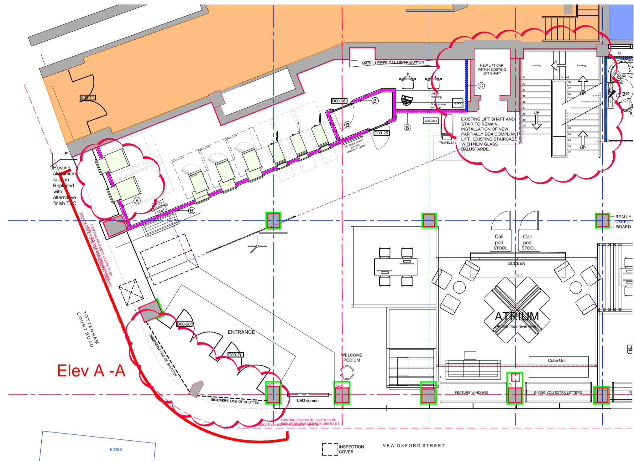
PROPOSED PLAN @ 1:100
