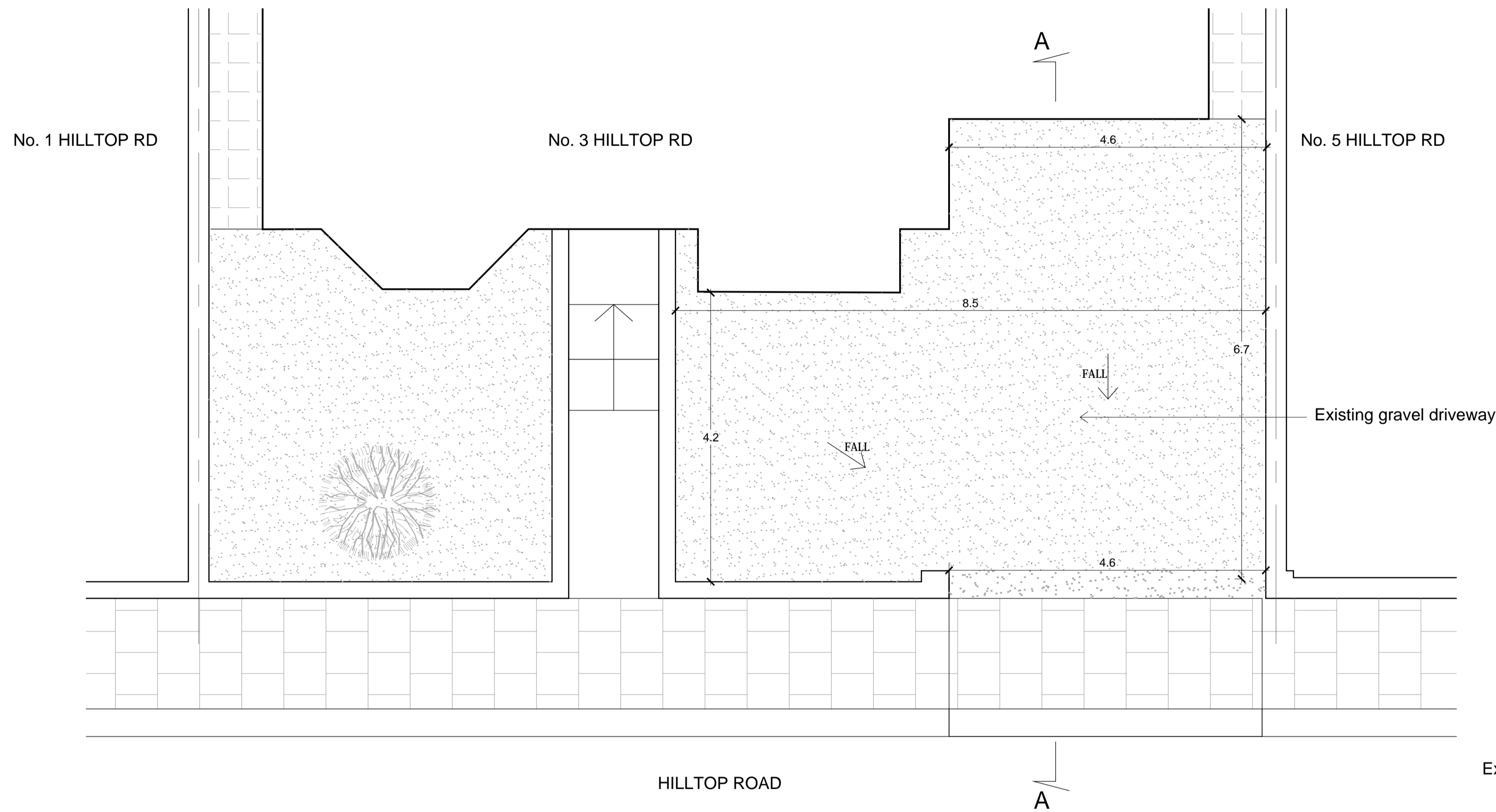
Existing Driveway Plan scale 1:50
