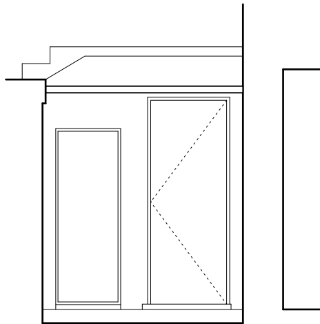
EXISTING FRONT AREA ARRANGEMENT - SIDE ELEVATION (RAILINGS/BALUSTRADING OMITTED FOR CLARITY)
