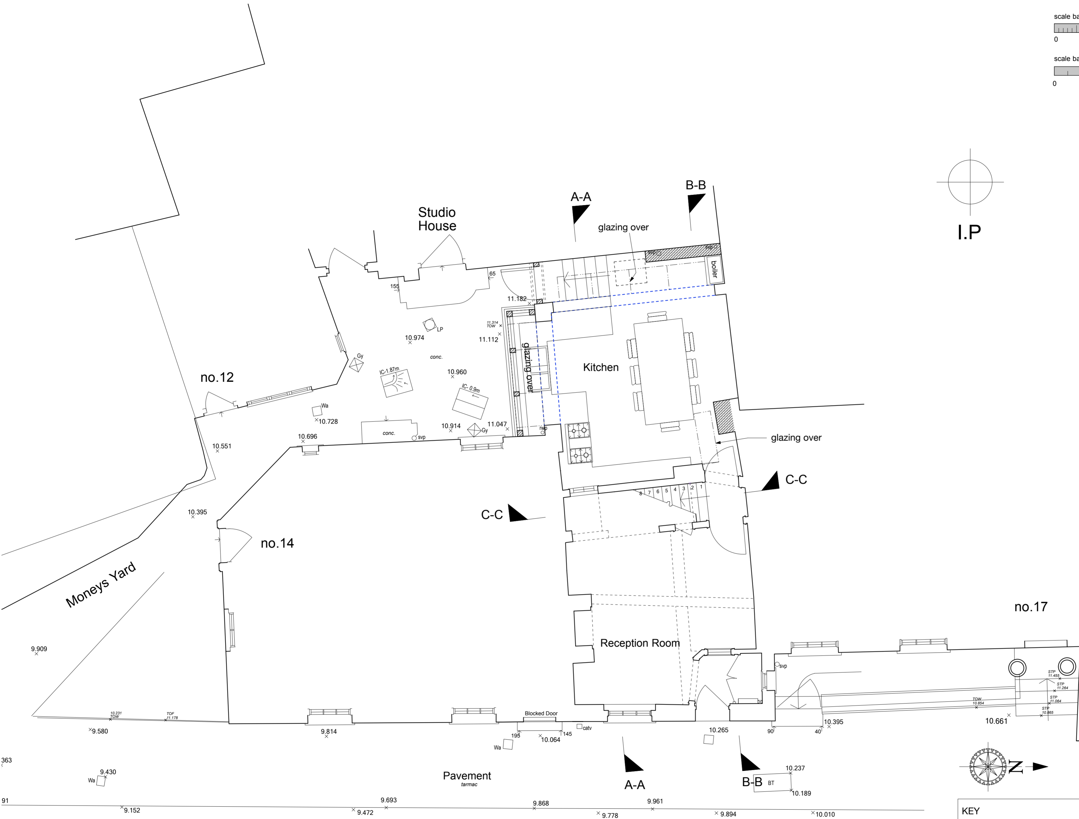
GROUND FLOOR PLAN Road - The Mount
