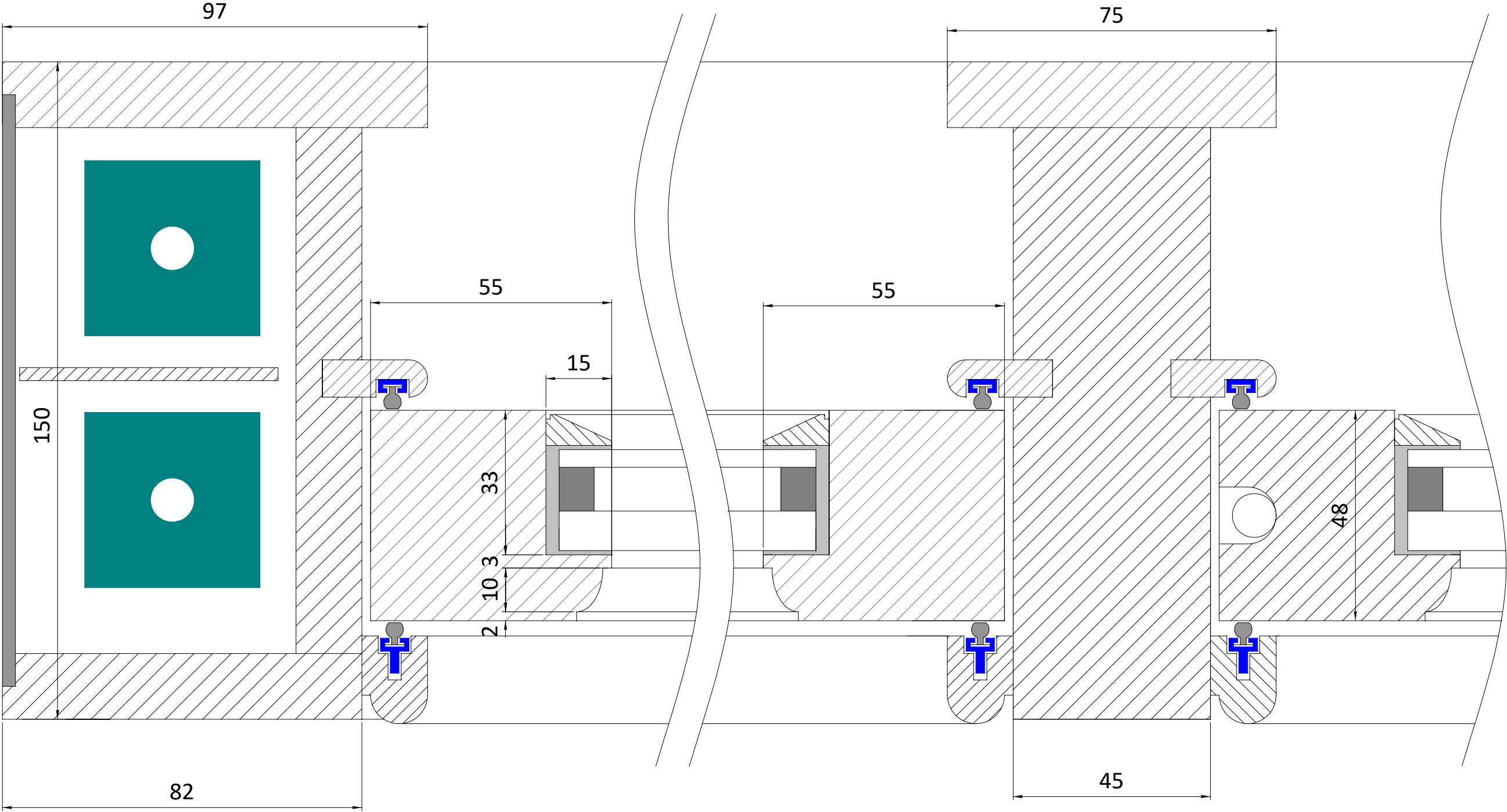
SECTION THROUGH FRAME JAMB AND MULLION - SCALE 1:1
