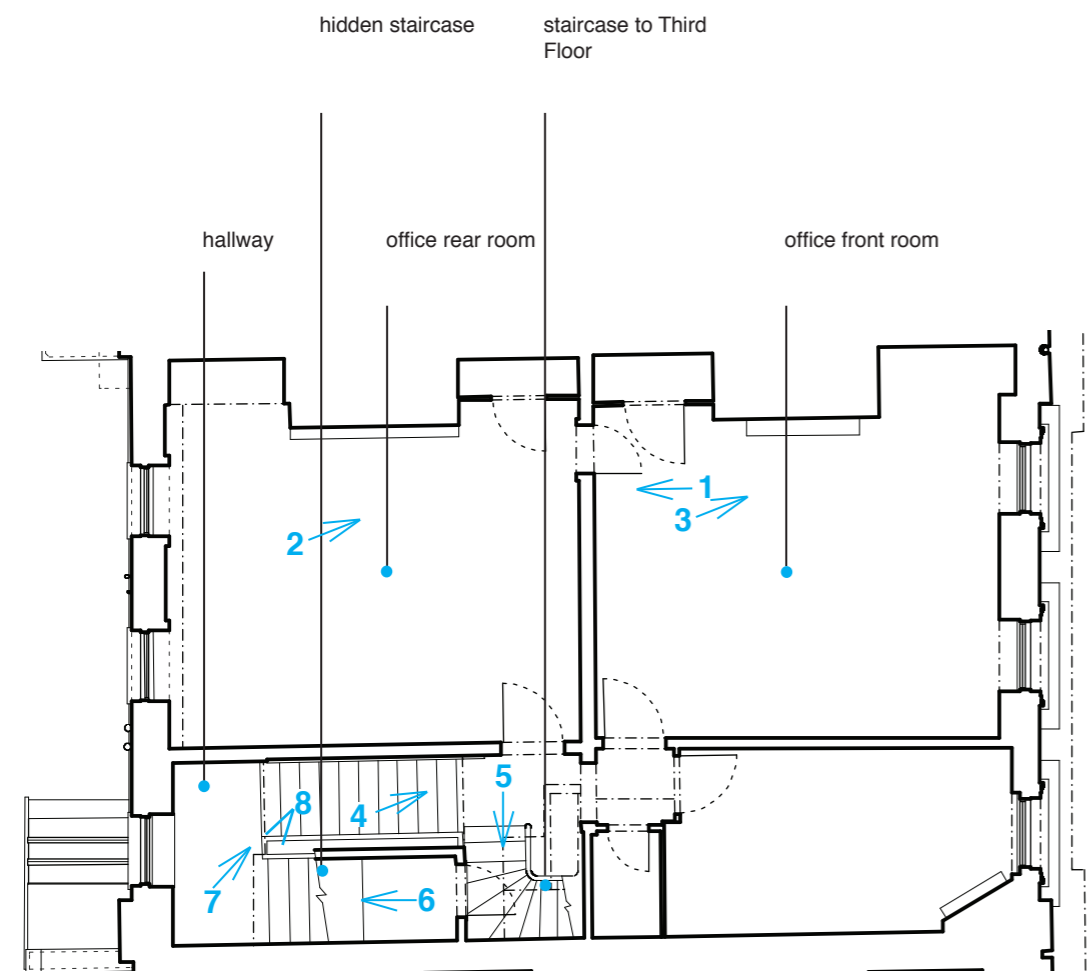
Existing Second Floor Plan
