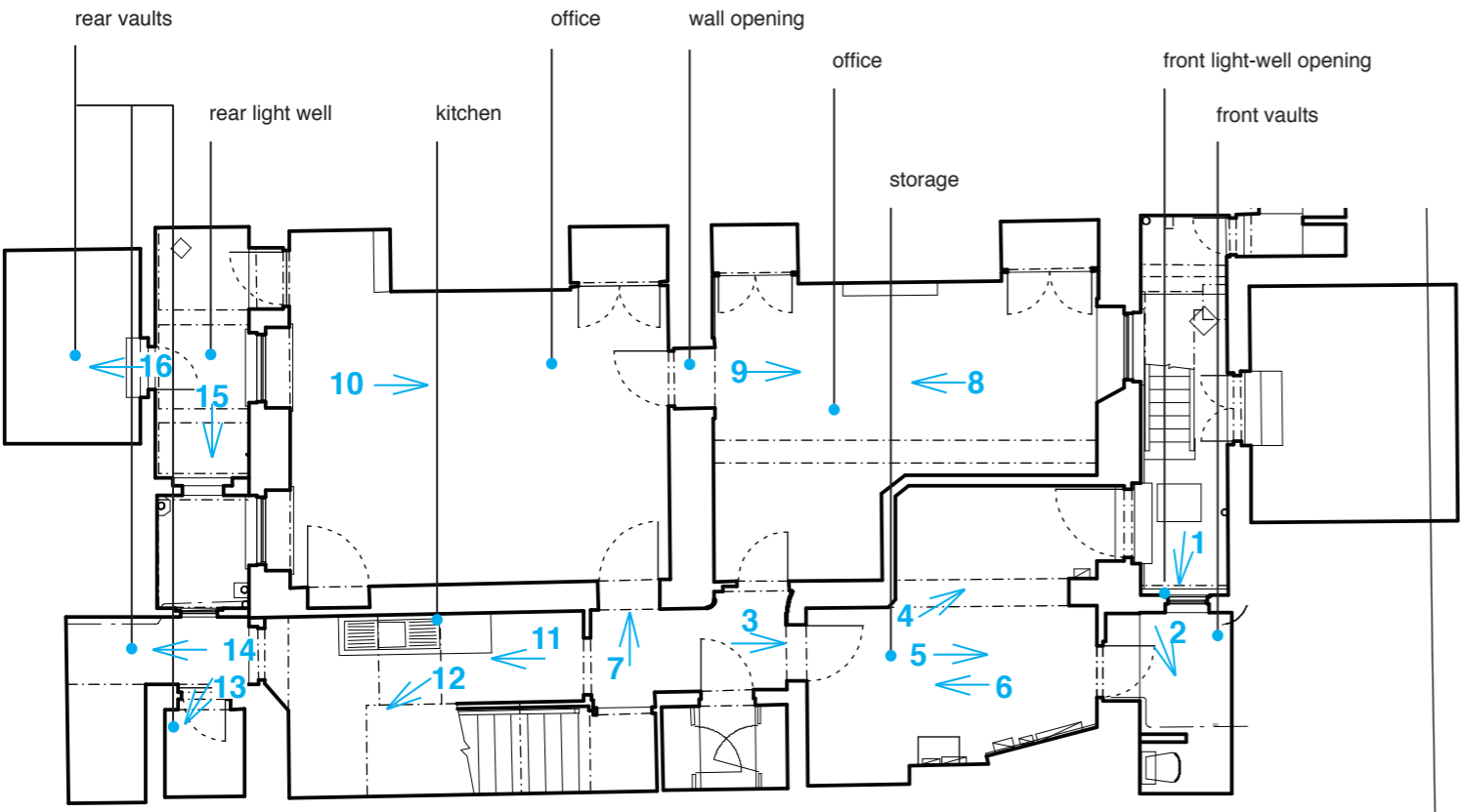
Existing Lower Ground Floor Plan
