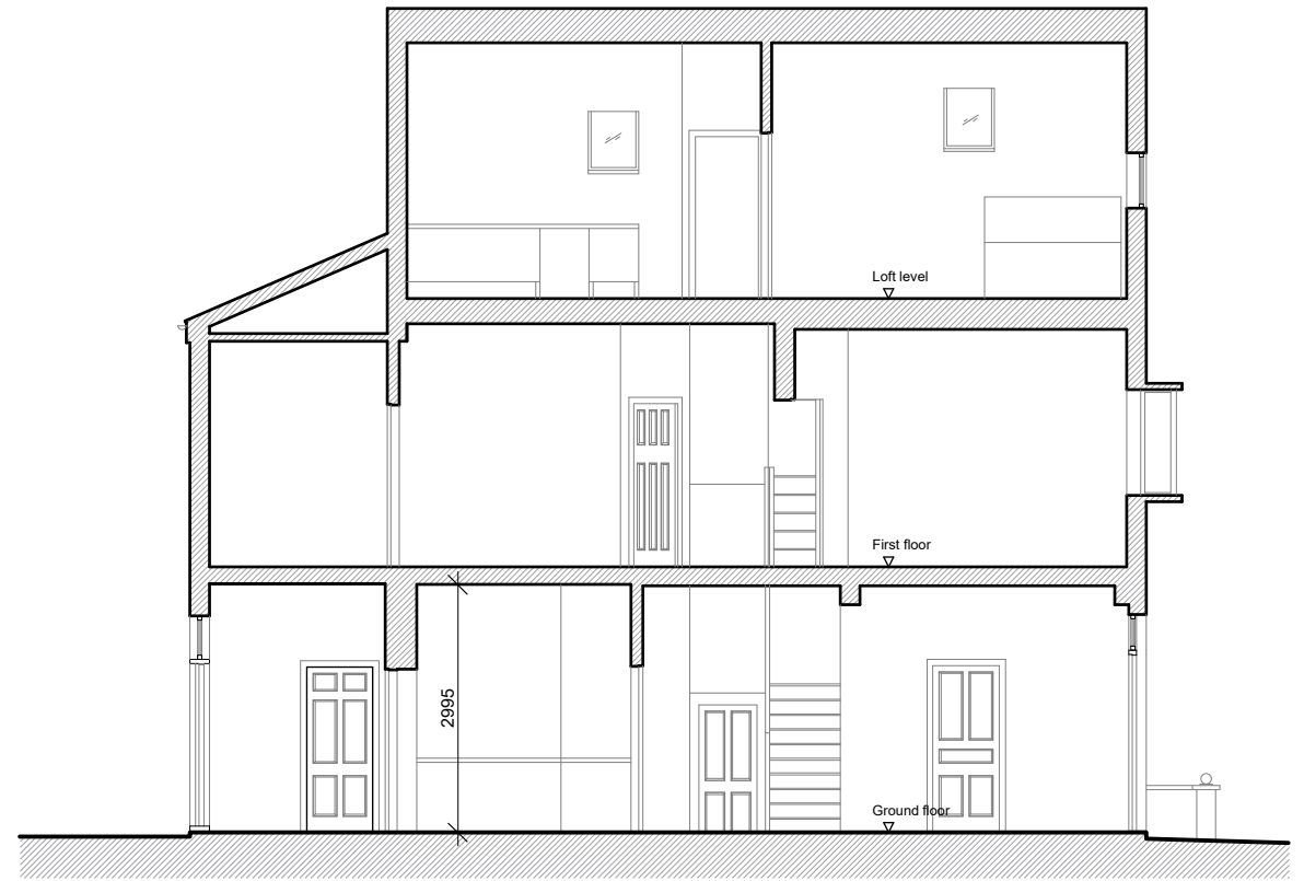
2 Section - Existing 1:100
