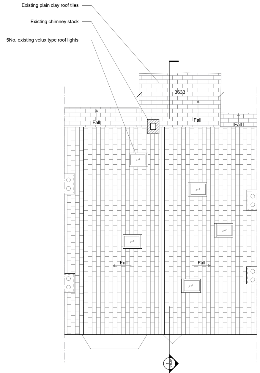
1 Roof plan - Existing 1:100
