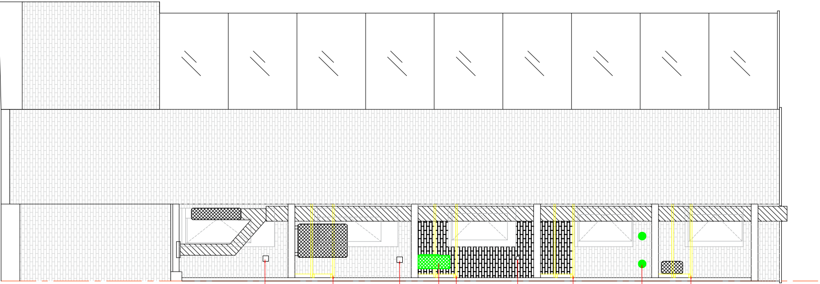
REAR ELEVATION 1:100 @ A3
