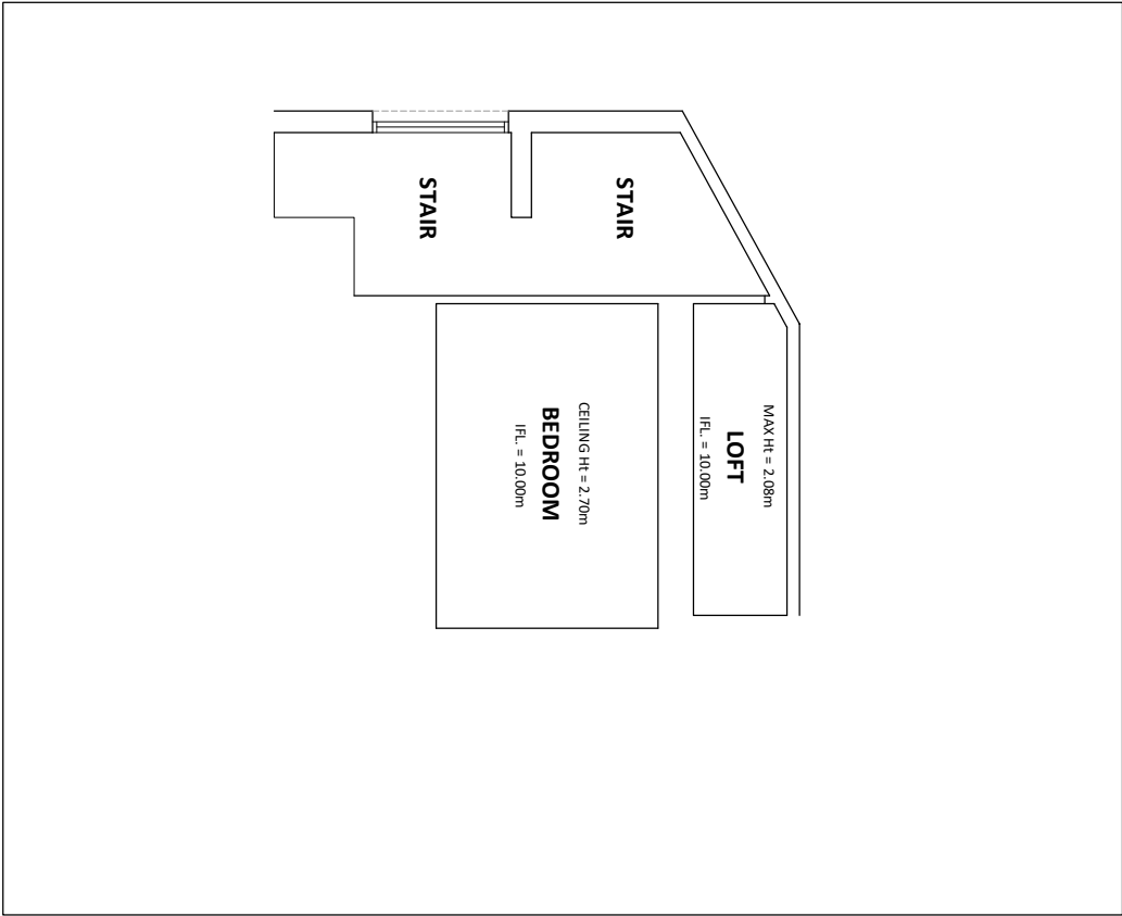
EXISTING SHORT-SECTION B-B
