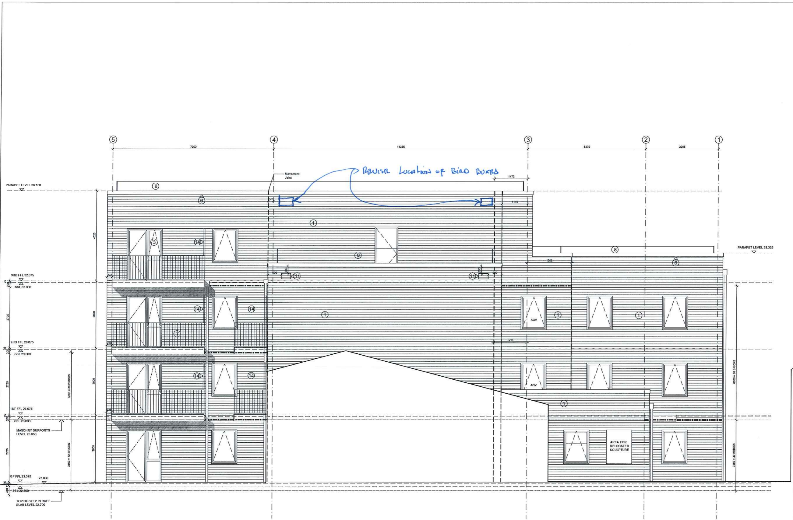
Proposed East Elevation Scale 1:50
