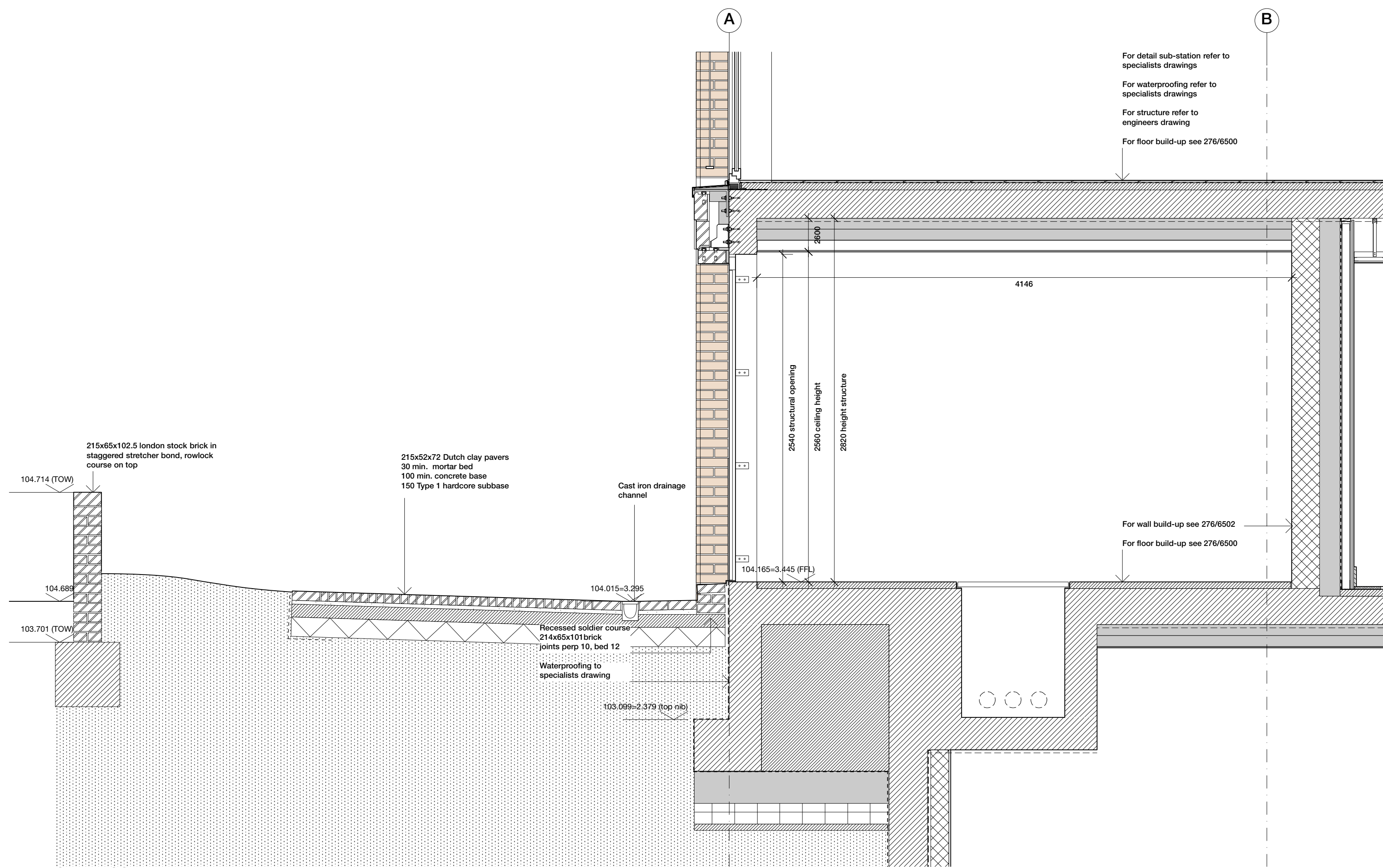
Section QQ
