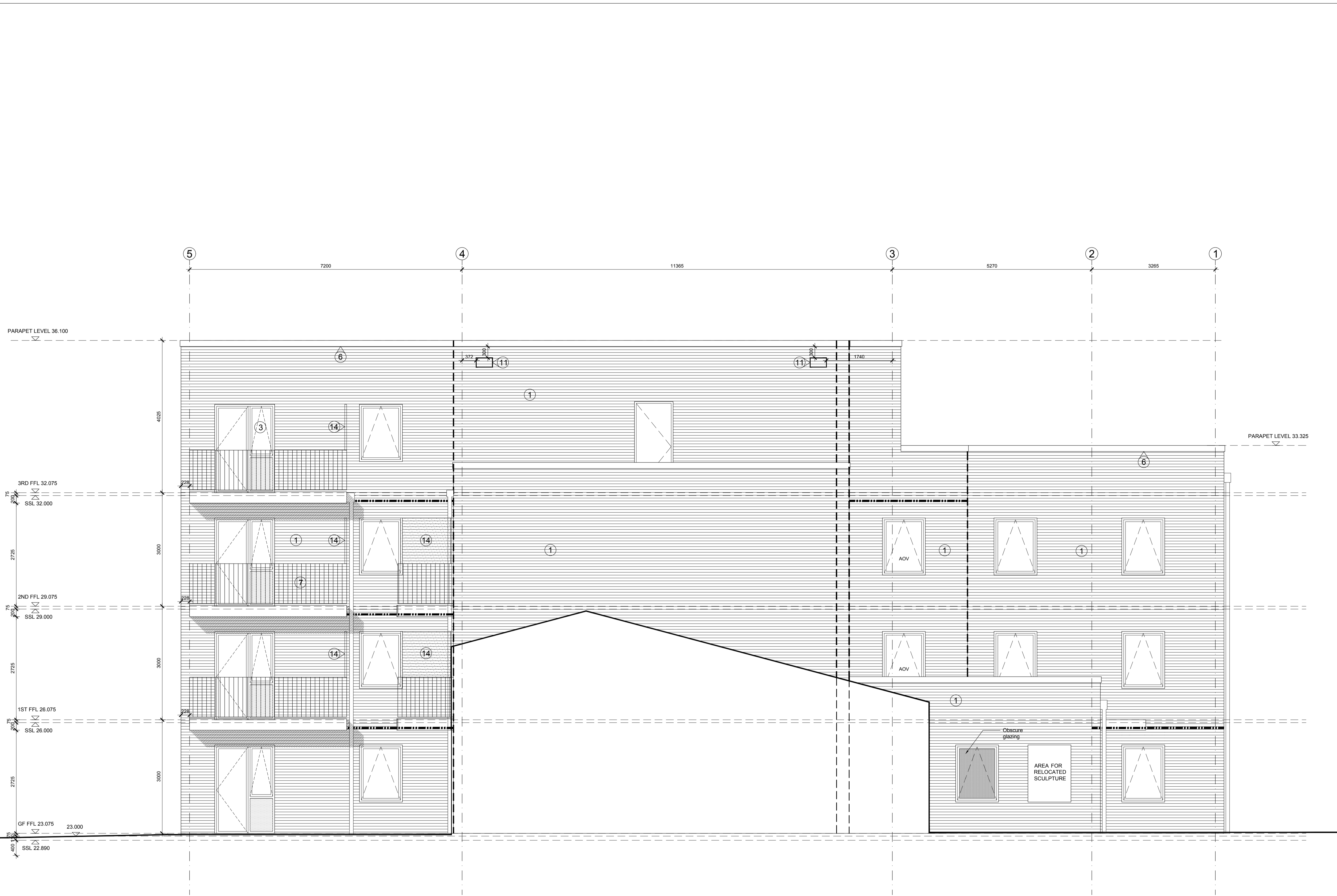
Proposed East Elevation Scale 1:50
