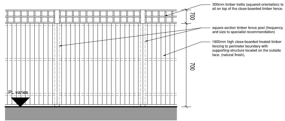
PROPOSED CLOSE-BOARDED TIMBER FENCE DETAIL (SECTION F)
