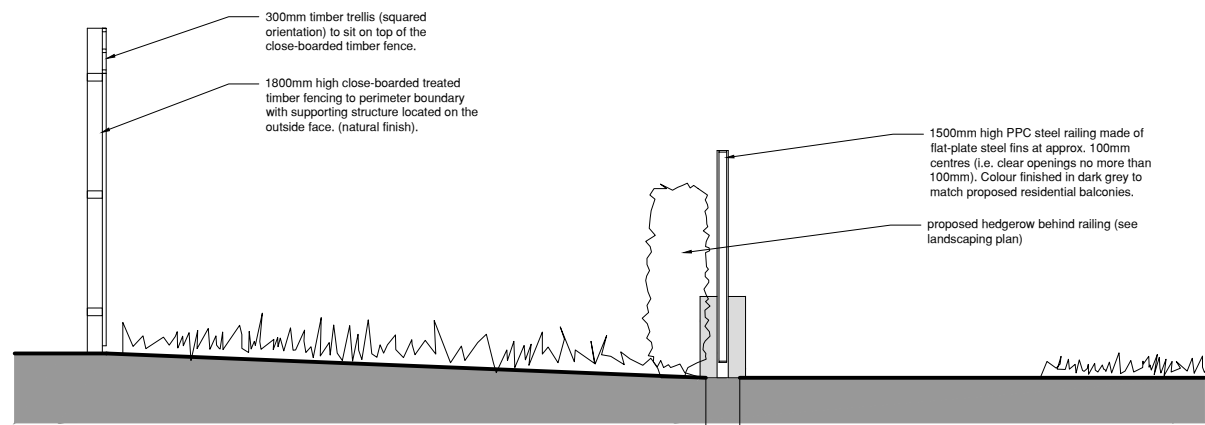
PROPOSED BOUNDARY TIMBER FENCE & STEEL RAILING ARRANGEMENT (SECTION E)
