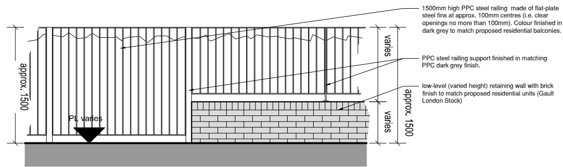
PROPOSED STEEL RAILING DETAIL (SECTION F)
