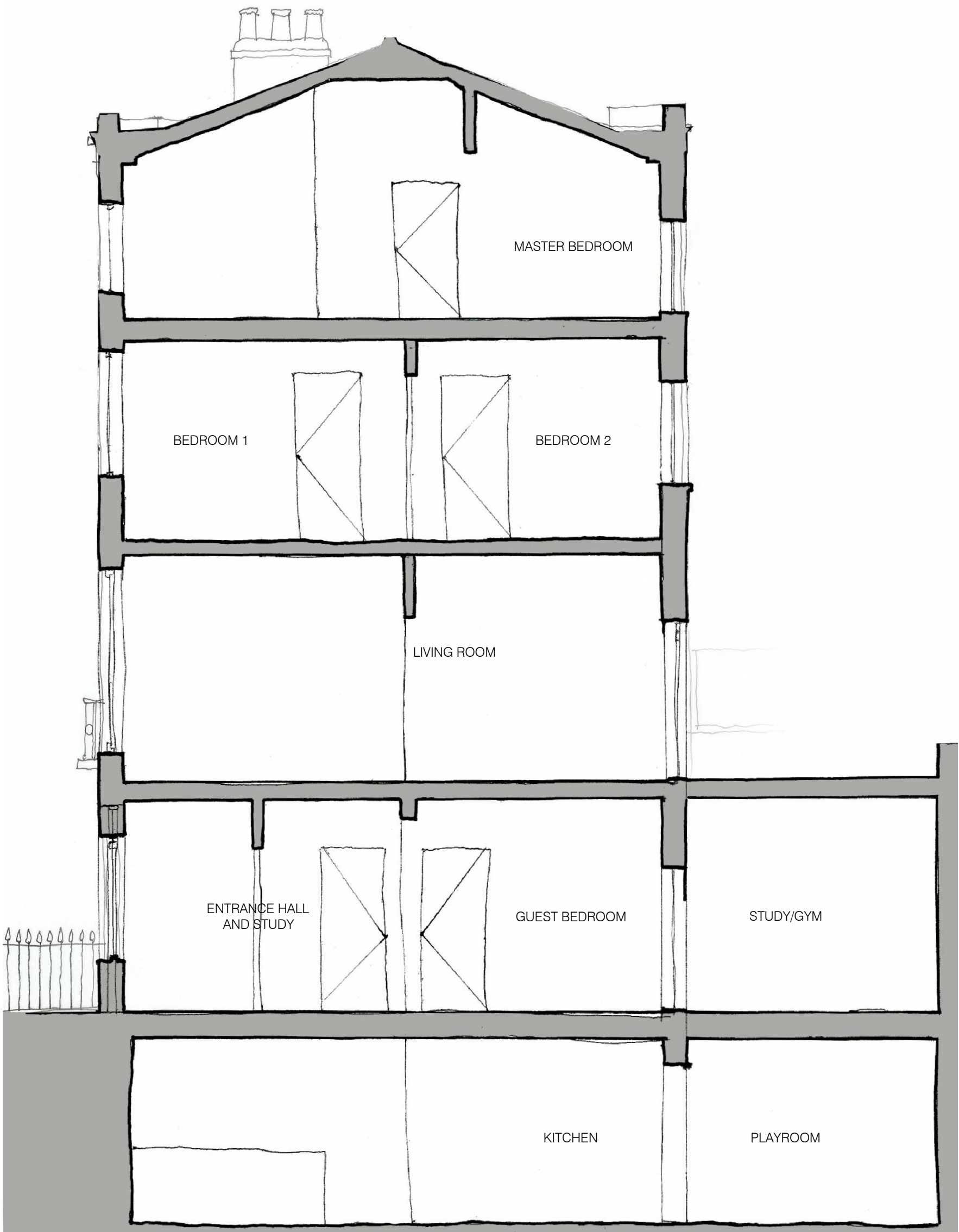
01 PROPOSED SECTION scale 1:50
