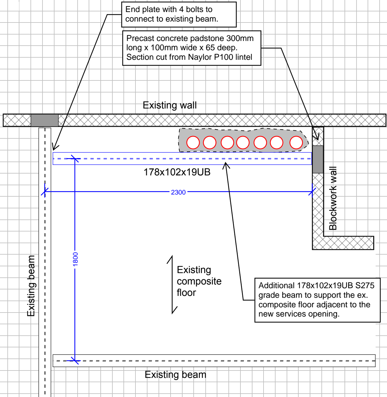
Remedial works - additional floor beam
