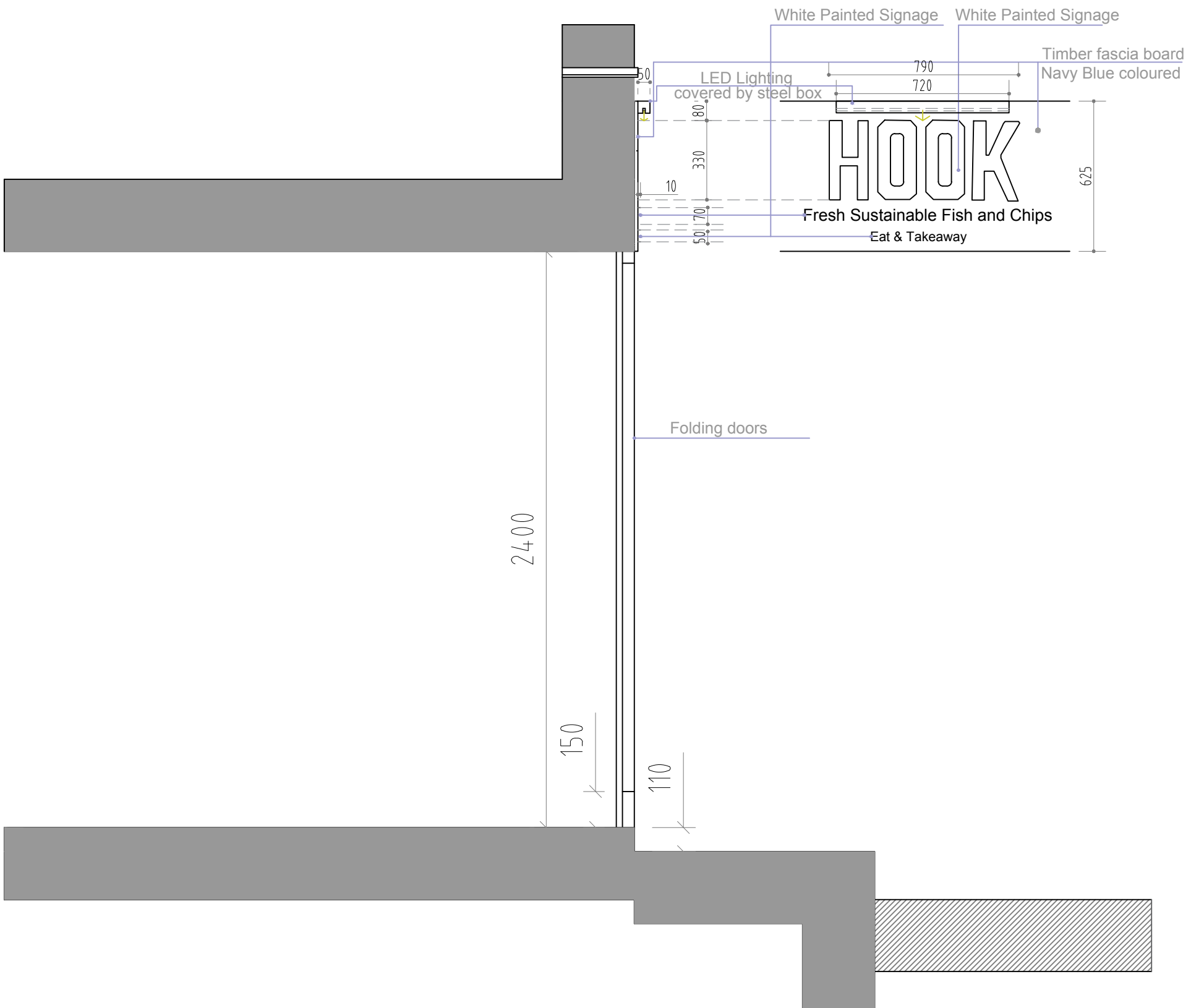
Section A
