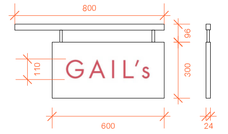
SIGNAGE NO. 1 + 2 PROPOSED HIGH LEVEL PROJECTING SIGN BOARD
