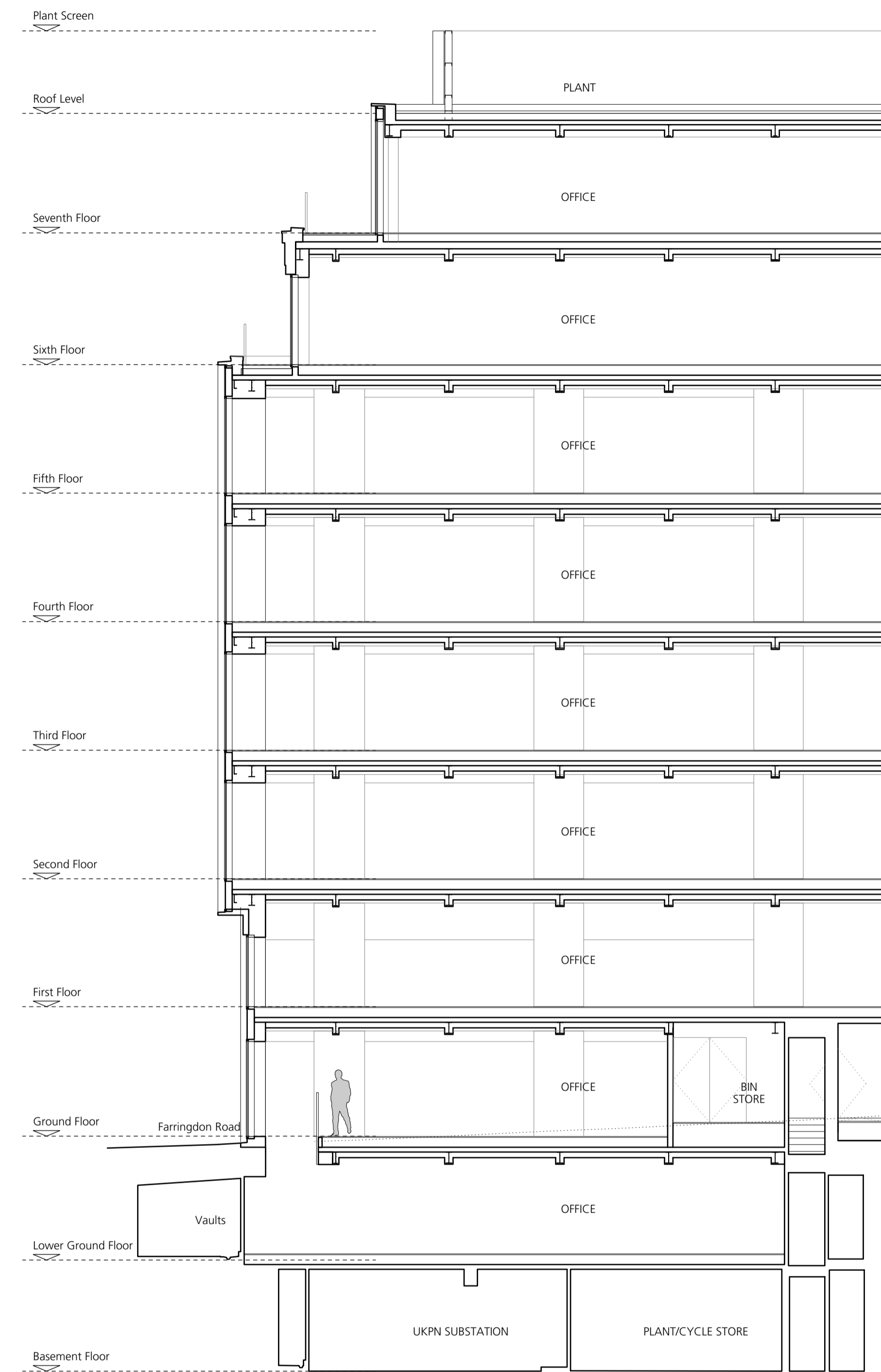
2 Proposed Section BB Scale: 1:100
