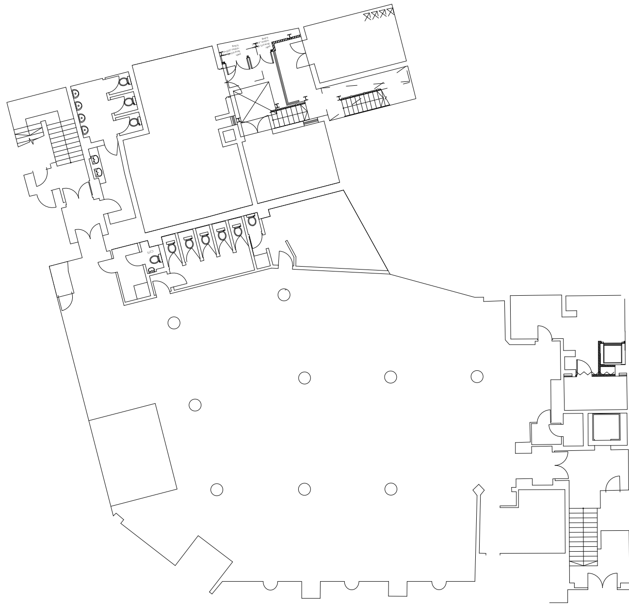
3 EXISTING BASEMENT PLAN 1:100 @ A1/1:200 @ A3
