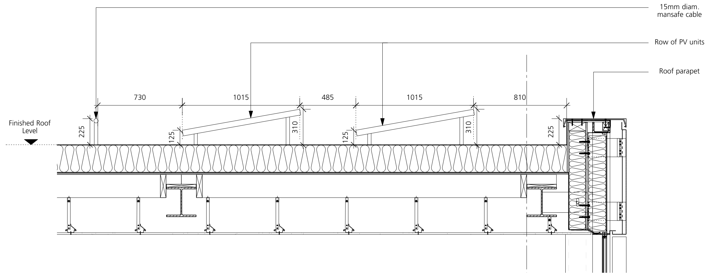
Back Hill Roof Section (As Built)
