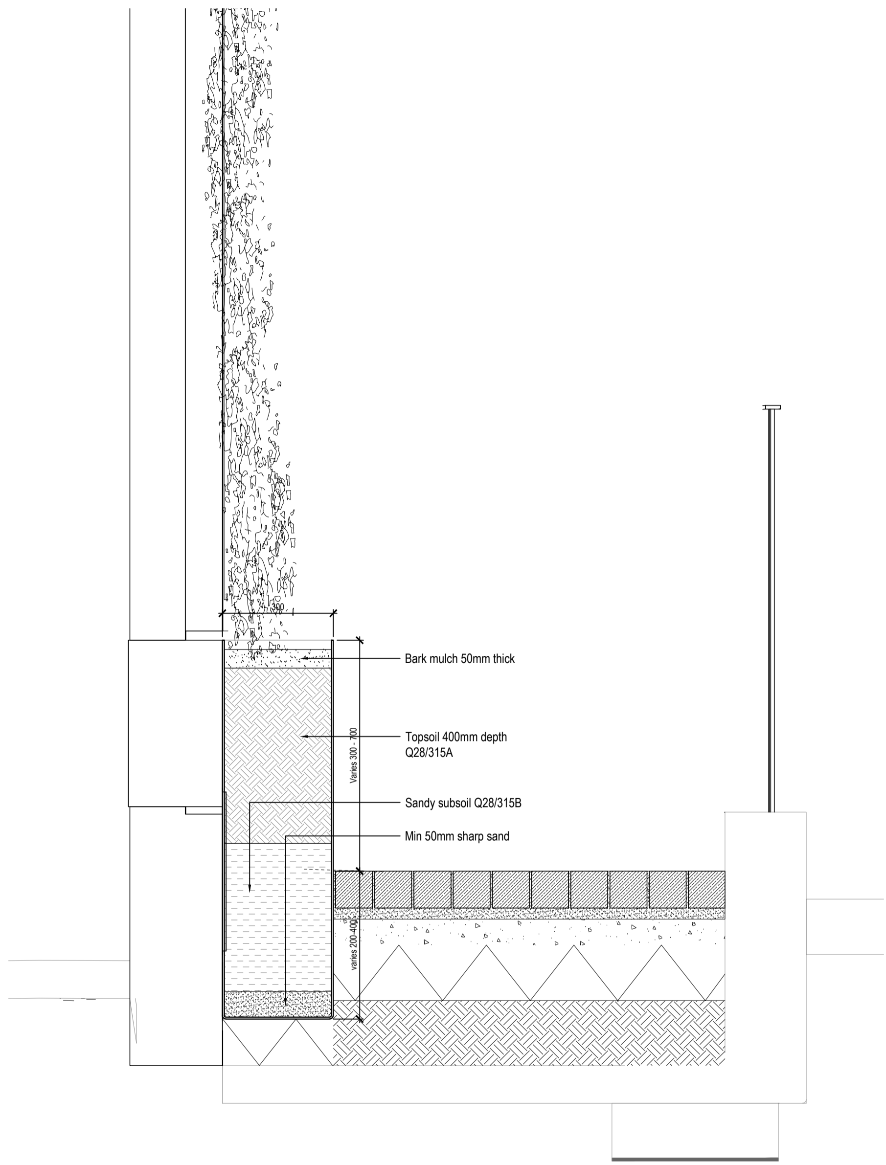
1 PLANTER TYPE PL1 - SECTION Scale 1: 10 @A1
