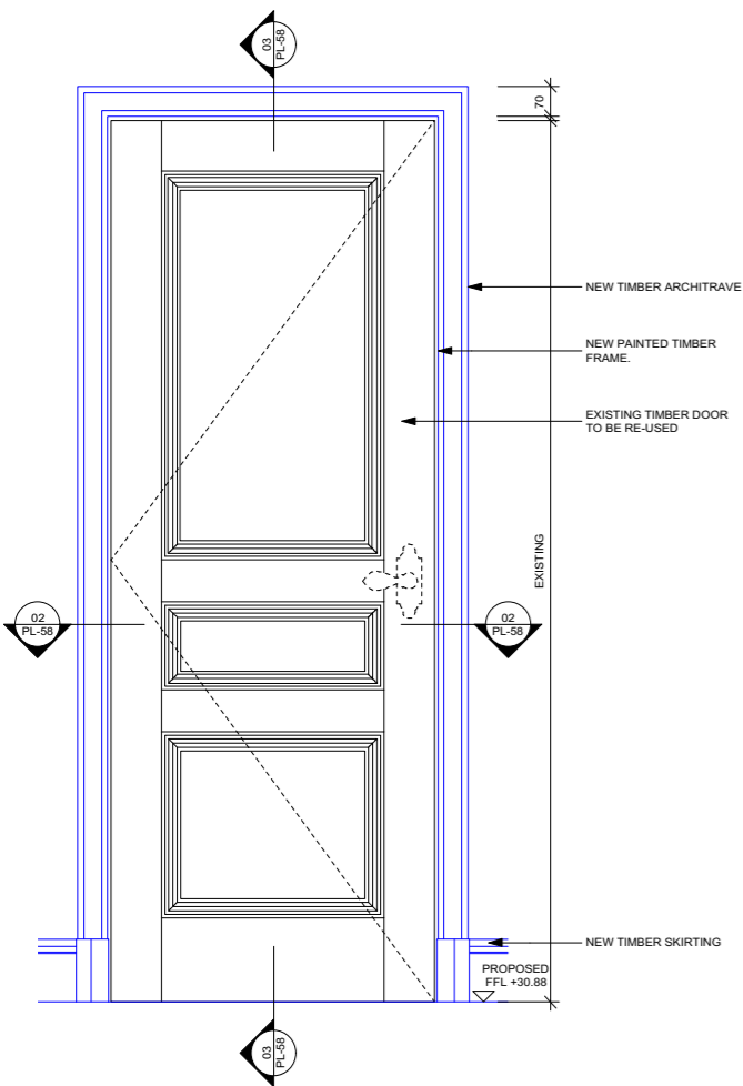
01 INTERNAL DOOR SCALE 1:10 ELEVATION PL-58
