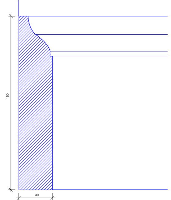
06 BOH SKIRTING PROFILE SCALE 1:1 PL-58
