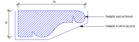
07 BOH ARCHITRAVE PROFILE SCALE 1:1 PL-58
