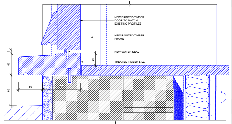
06 DOOR DL18 SCALE 1:2 HEAD & THRESHOLD DETAIL PL-55
