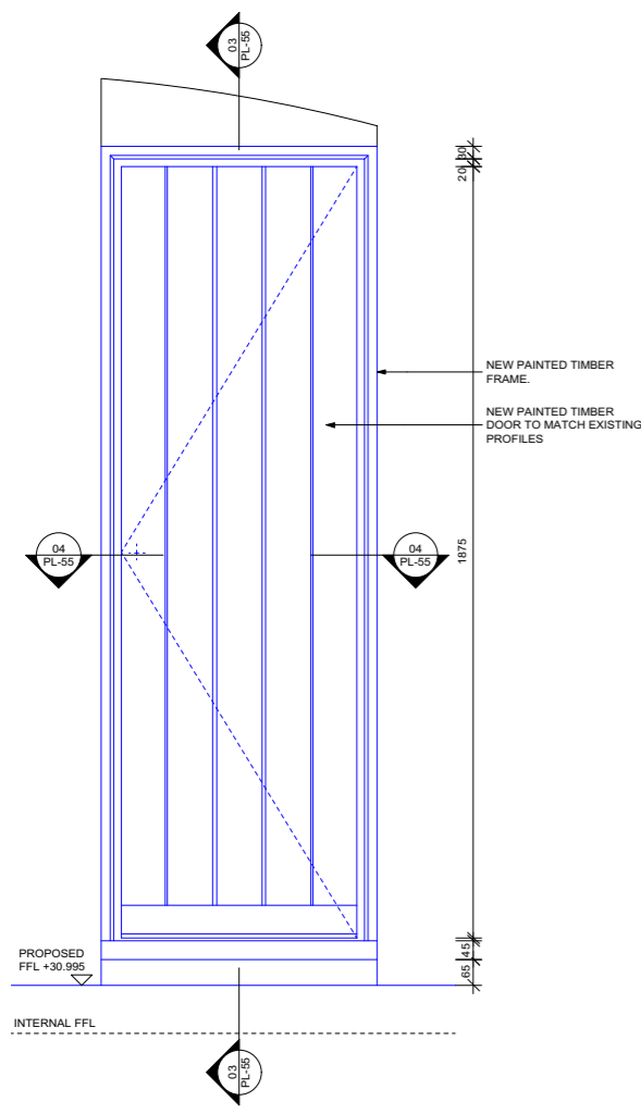
1 DOOR DL18 SCALE 1:10 EXTERNAL ELEVATION PL-55
