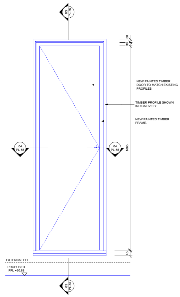
02 DOOR DL18 SCALE 1:10 INTERNAL ELEVATION PL-55
