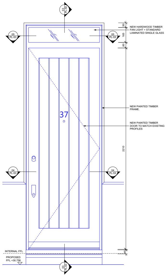
1 REAR DOOR DL02 SCALE 1:10 EXTERNAL ELEVATION PL-53
