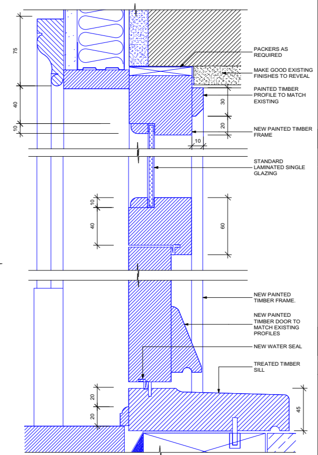
07 REAR DOOR DL02 SCALE 1:2 HEAD & THRESHOLD DETAIL PL-53
