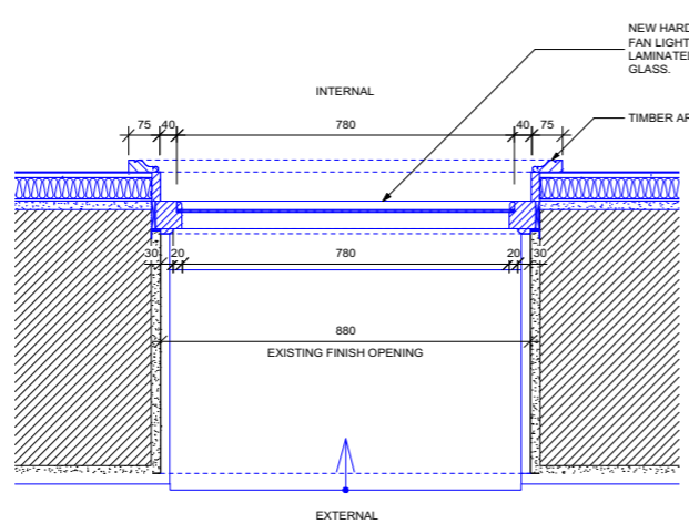
05 REAR DOOR DL02 SCALE 1:10 PLAN PL-53
