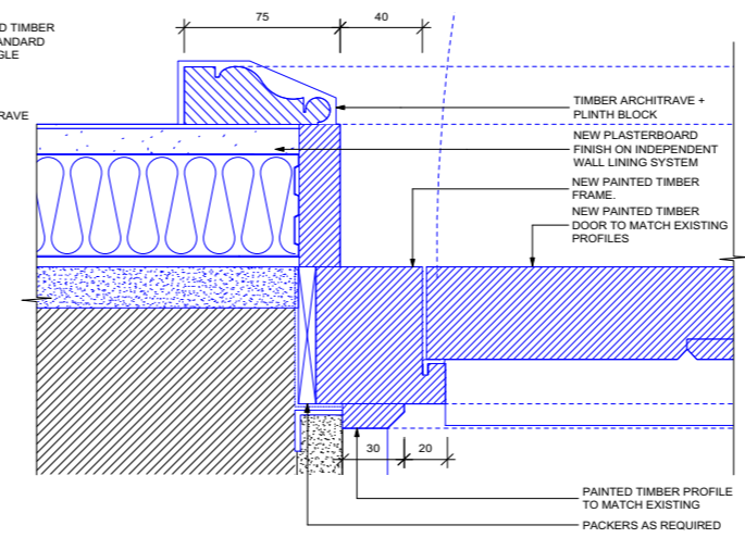
06 REAR DOOR DL02 SCALE 1:2 JAMB DETAIL PL-53
