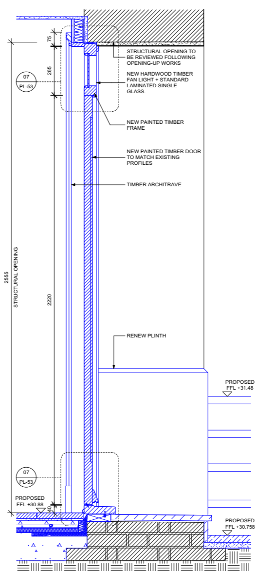
03 REAR DOOR DL02 SCALE 1:10 SECTION PL-53
