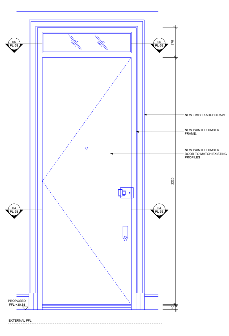
02 REAR DOOR DL02 SCALE 1:10 INTERNAL ELEVATION PL-53
