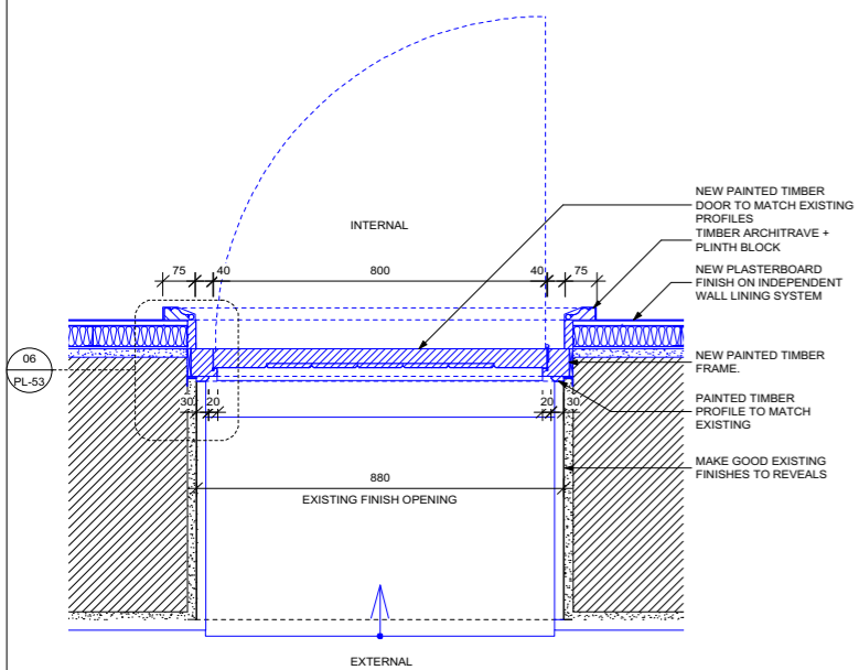
04 REAR DOOR DL02 SCALE 1:10 PLAN PL-53
