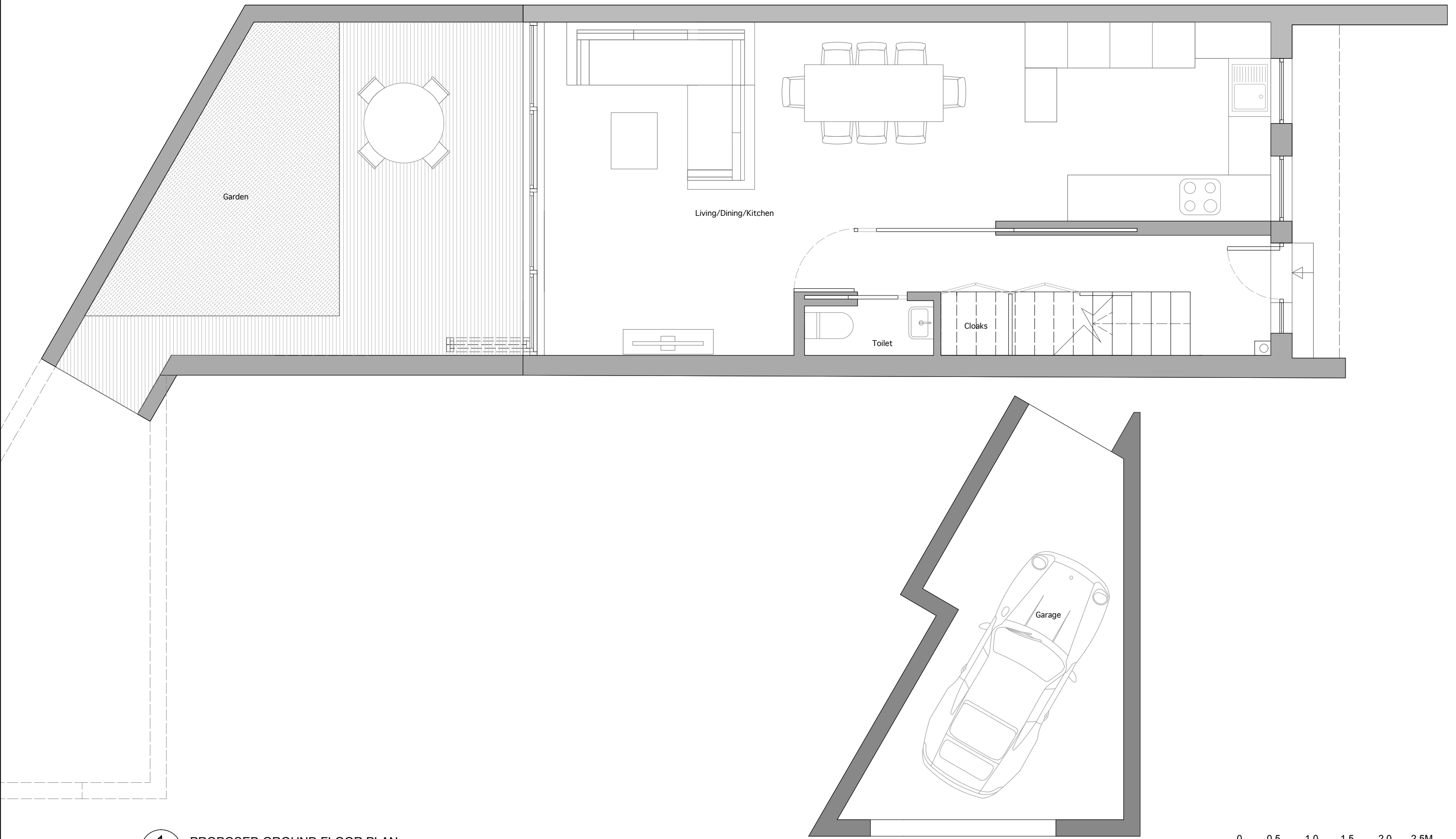
1 PROPOSED GROUND FLOOR PLAN 1:50
