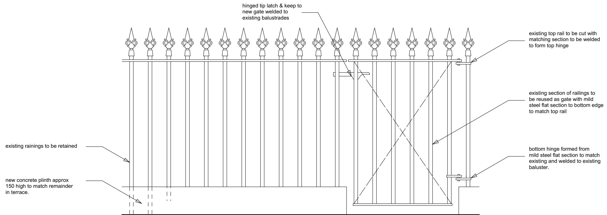
ELEVATION TO RAILINGS scale 1:10
