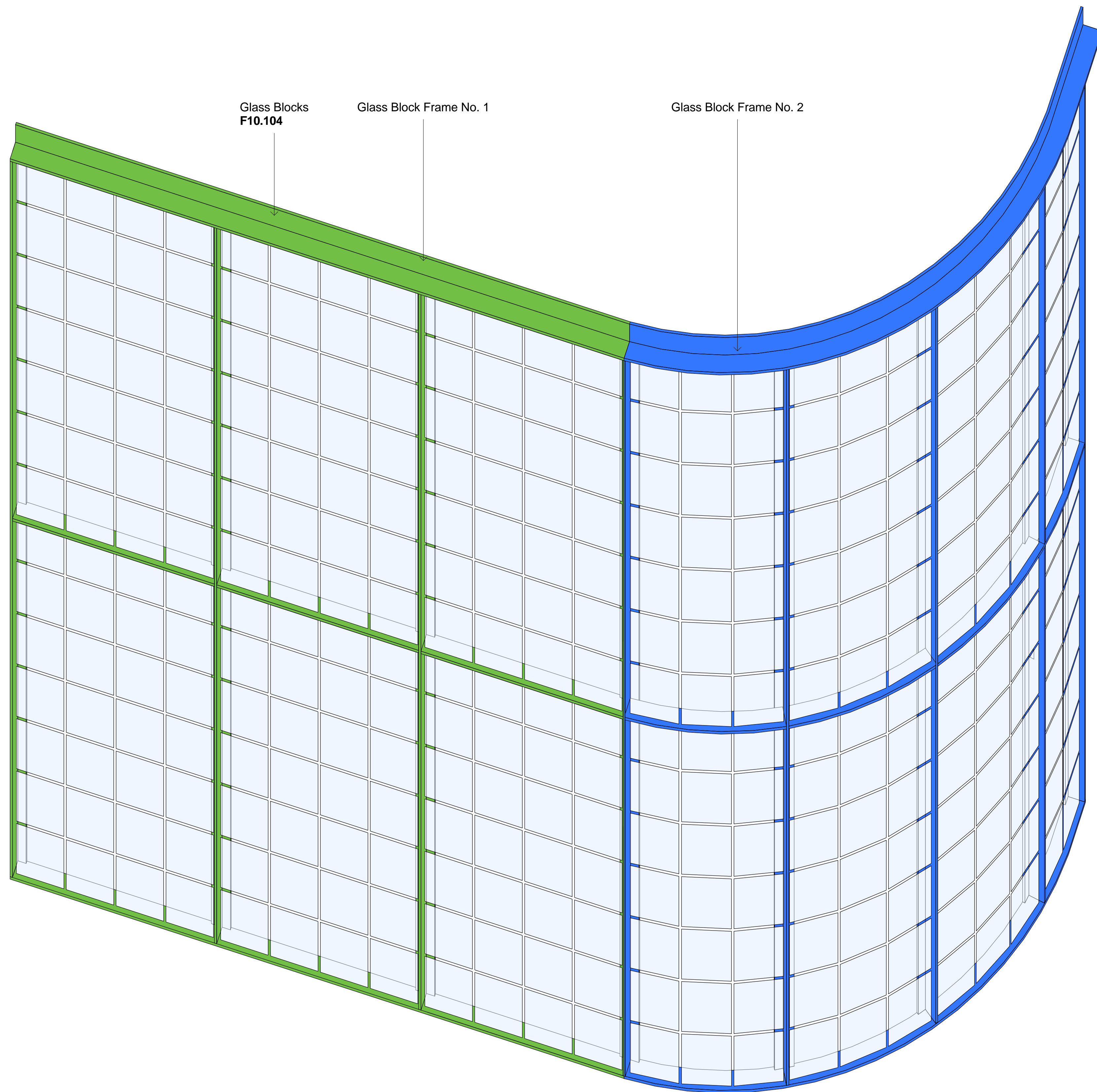
1 Glass Block Structure Scope Scale: 1 : 10
