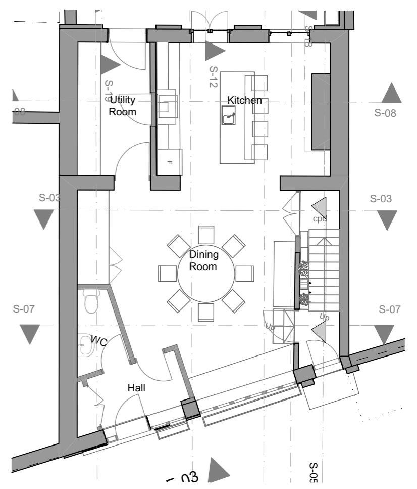
Ground Floor Plan 1:00
