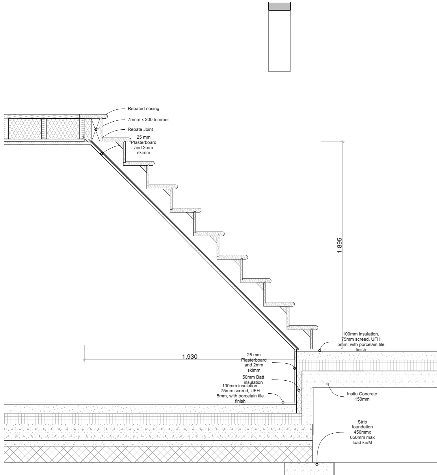
Stairs Building Section 1:20
