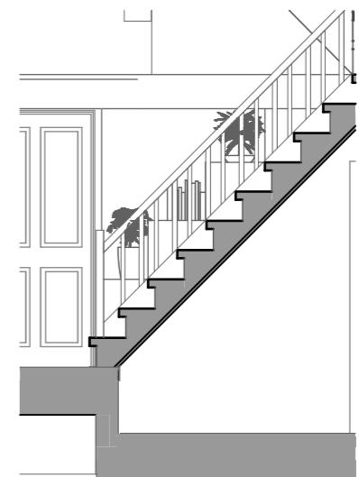
Stair section with stairs
