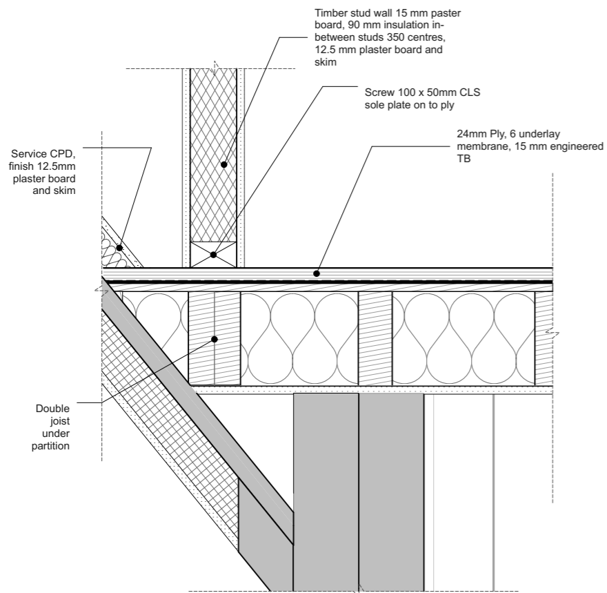
D-25 Detail 1:10
