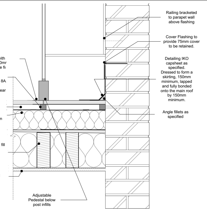
D-29 Detail 1:10
