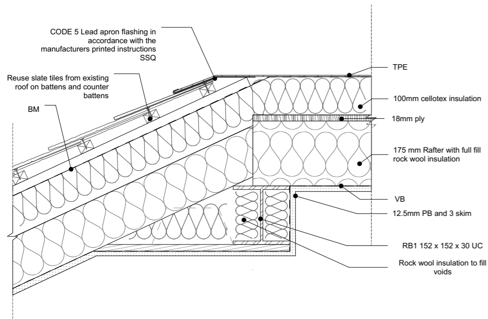
D-28 Detail 1:10
