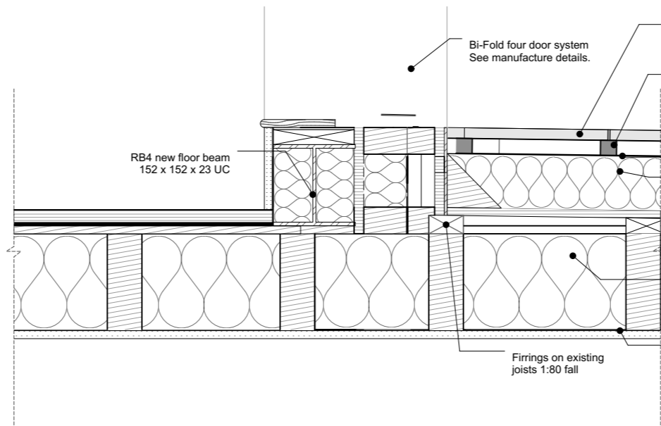
D-26 Detail 1:10
