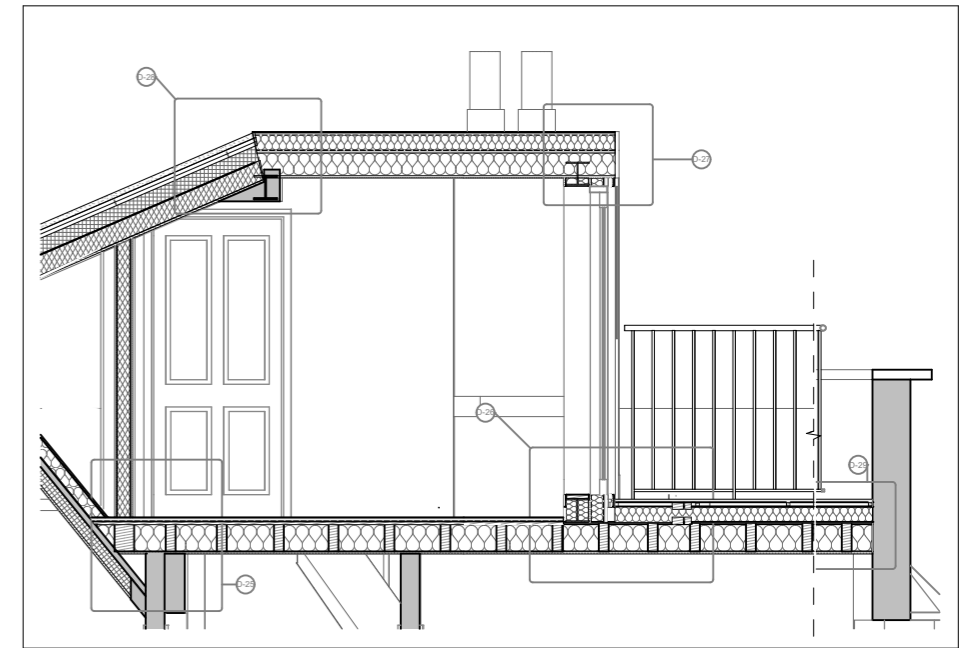
S-11 Detail Section- Extension 1:50
