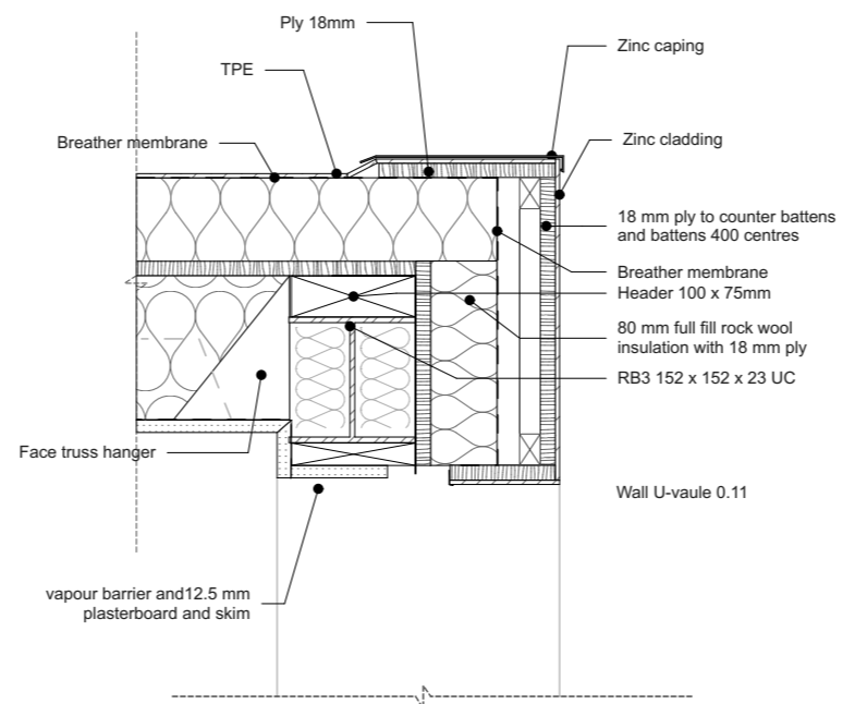
D-27 Detail 1:10
