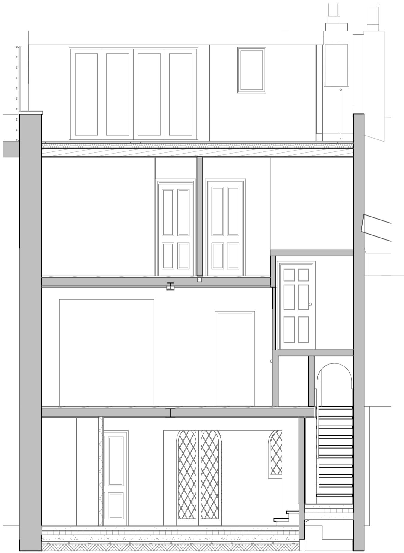
S-10 Building Section 1:50
